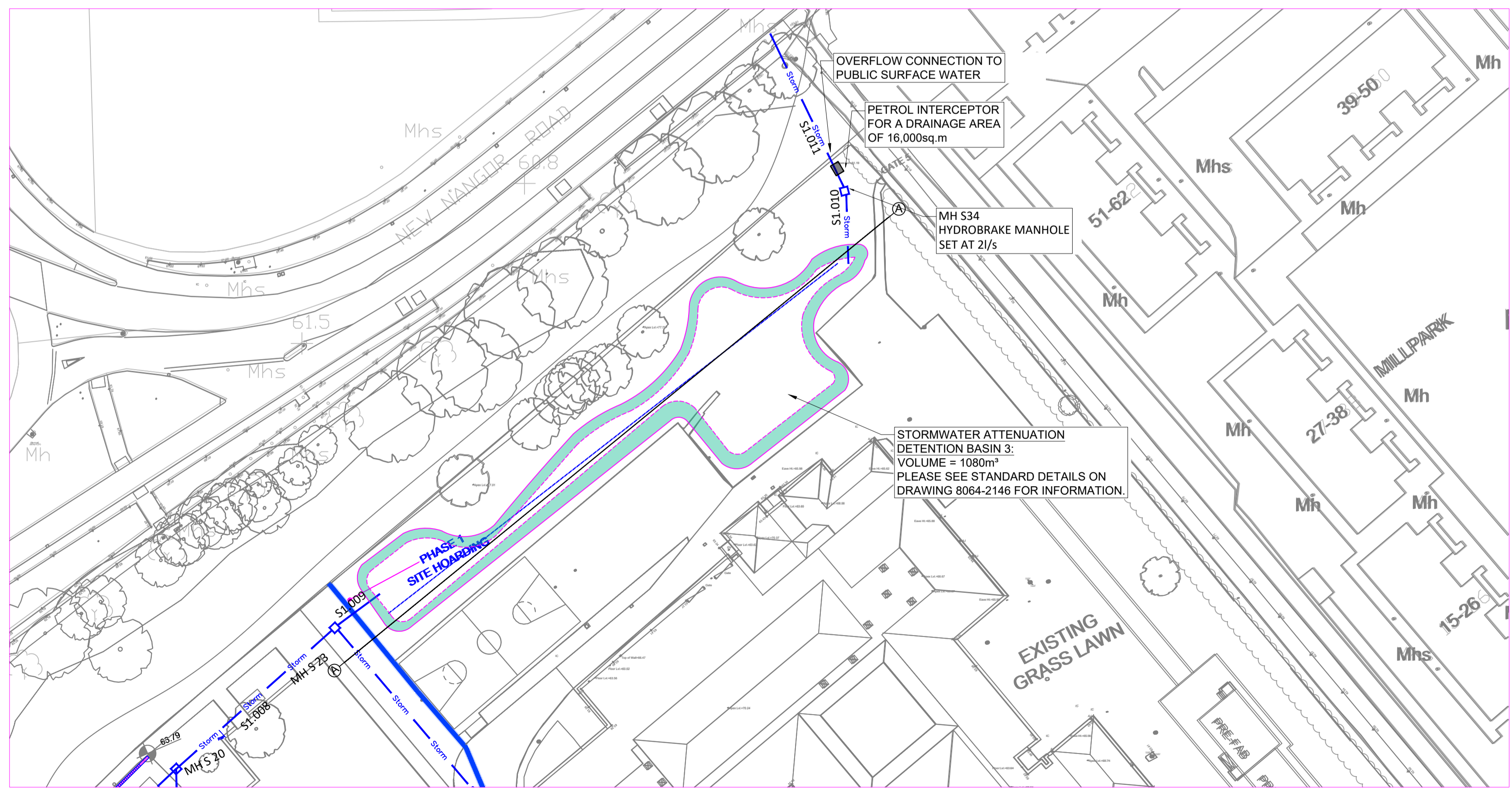
ATTENUATION TANK PLAN SCALE: 1:100
