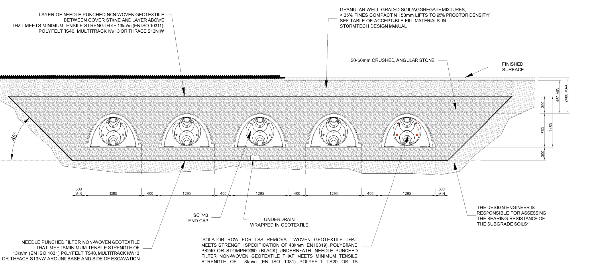
SECTION A - TANK D SCALE @ A1: 1:50 SCALE @ A3: 1:100
