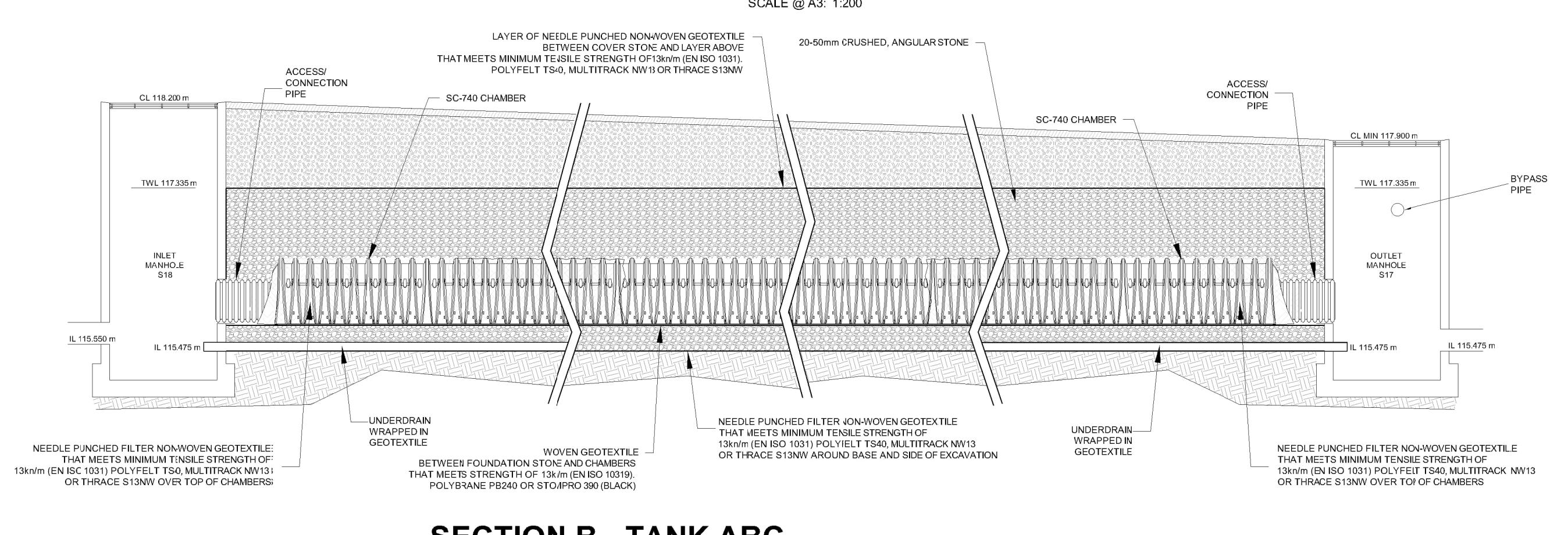
SECTION B - TANK ABC SCALE @ A1: 1:75 SCALE @ A3: 1:100
