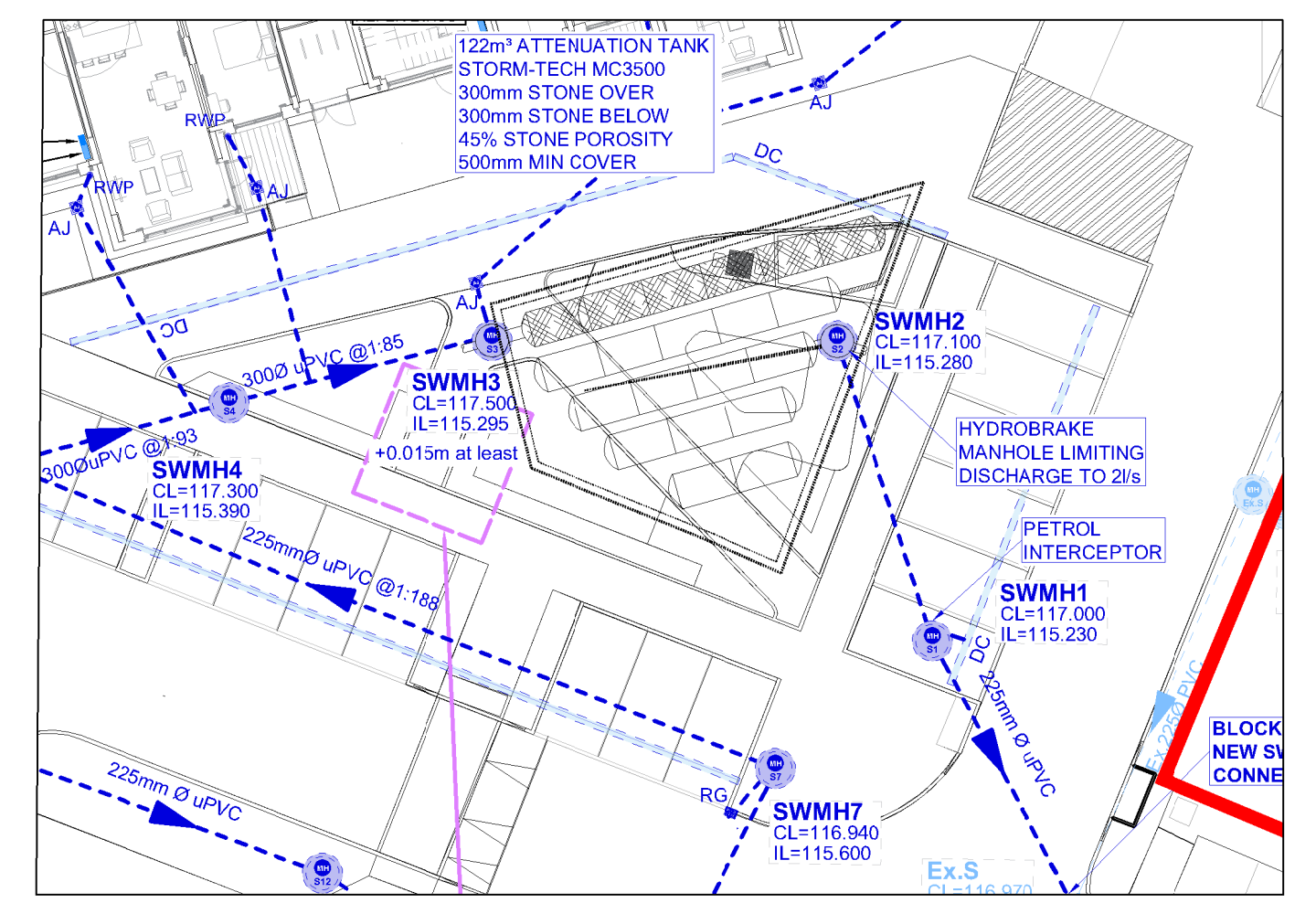
PROPOSED SURFACE WATER DRAINAGE LAYOUT - TANK D SCALE @ A1: 1:250 SCALE @ A3: 1:500
