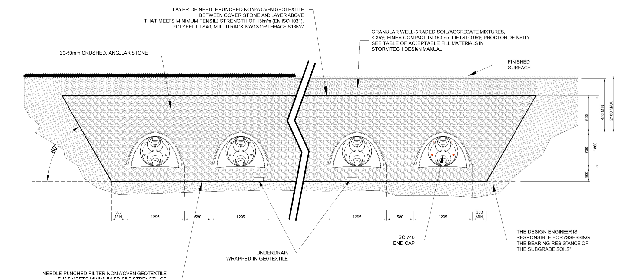
SECTION A - TANK ABC SCALE @ A1: 1:50 SCALE @ A3: 1:100
