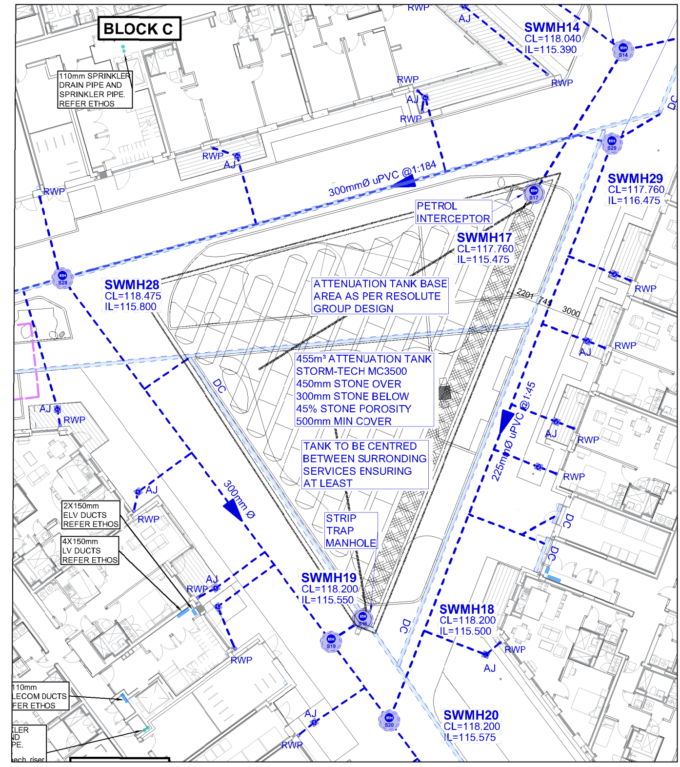
PROPOSED SURFACE WATER DRAINAGE LAYOUT - TANK ABC SCALE @ A1: 1:250 SCALE @ A3: 1:500
