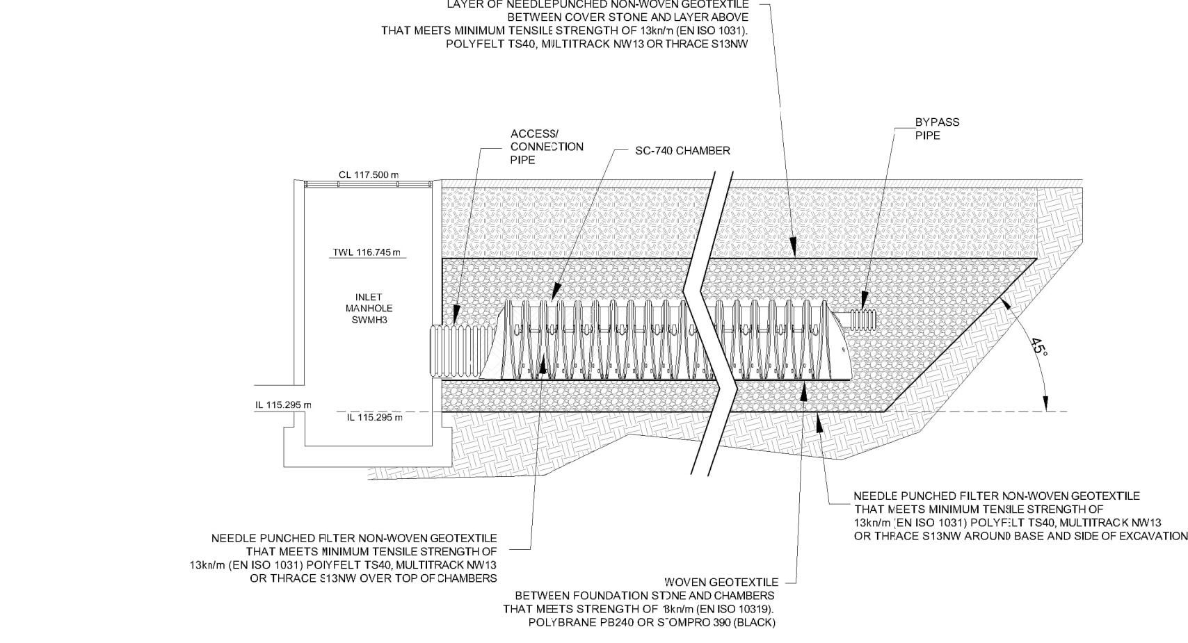
SECTION B - TANK D SCALE @ A1: 1:75 SCALE @ A3: 1:100
