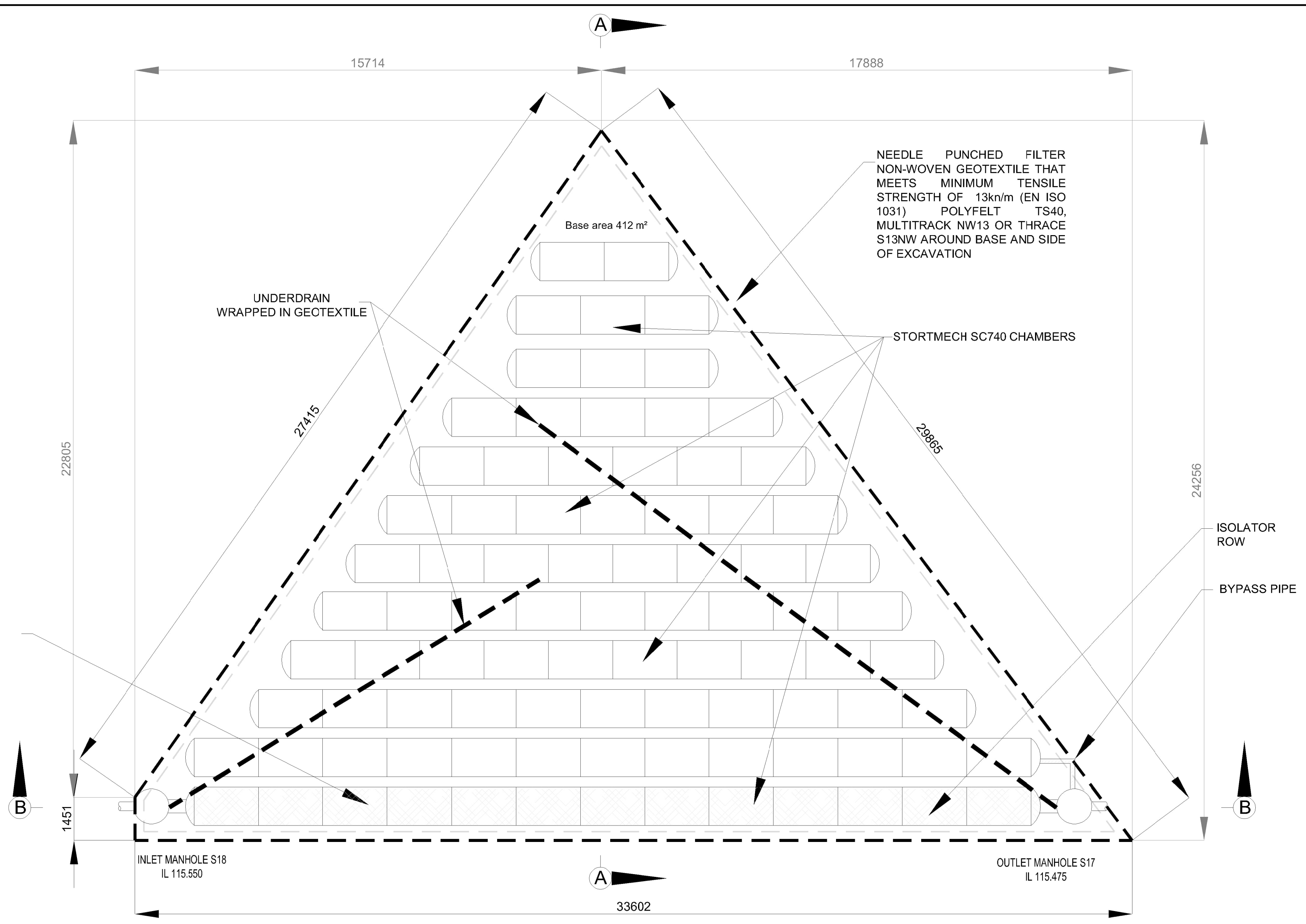
PLAN - TANK ABC SCALE @ A1: 1:100 SCALE @ A3: 1:300
