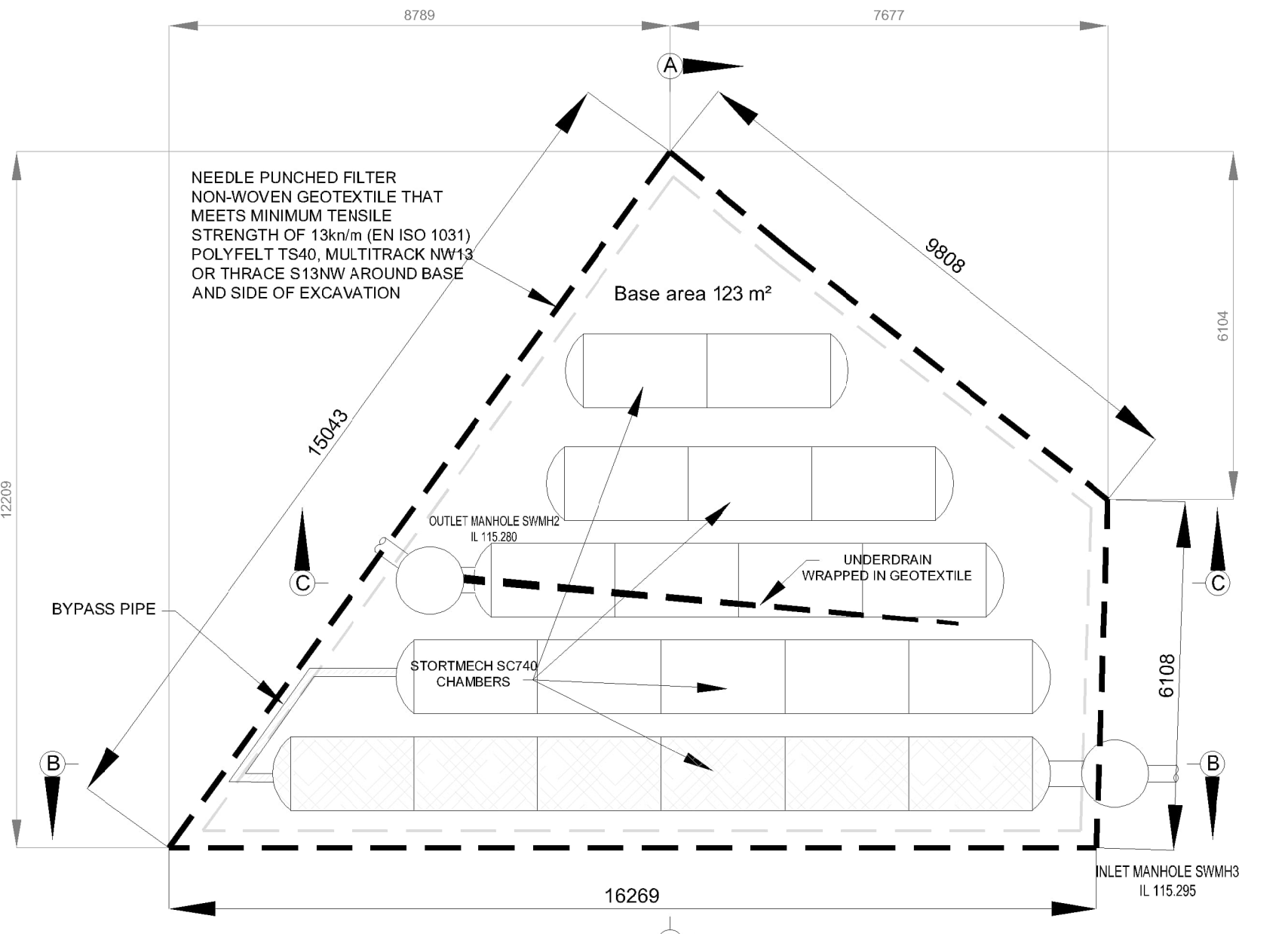
PLAN - TANK D SCALE @ A1: 1:100 SCALE @ A3: 1:200
