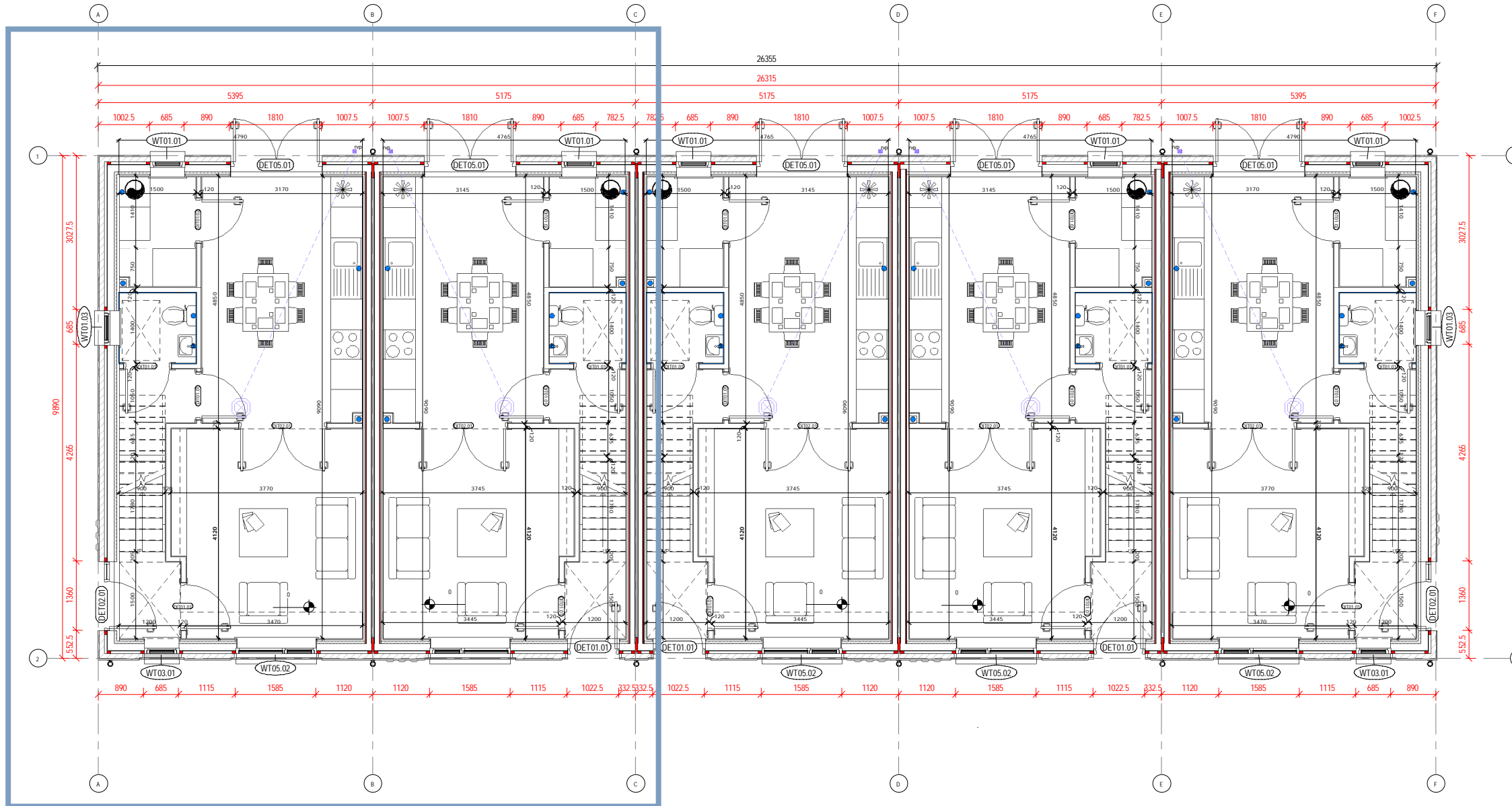
1 GROUND FLOOR PLAN Scale: 1:50
