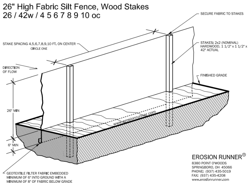
Figure 4- 1: Typical silt fence detail
