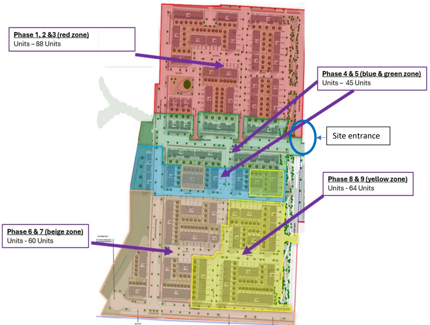
Construction Phasing Plan
