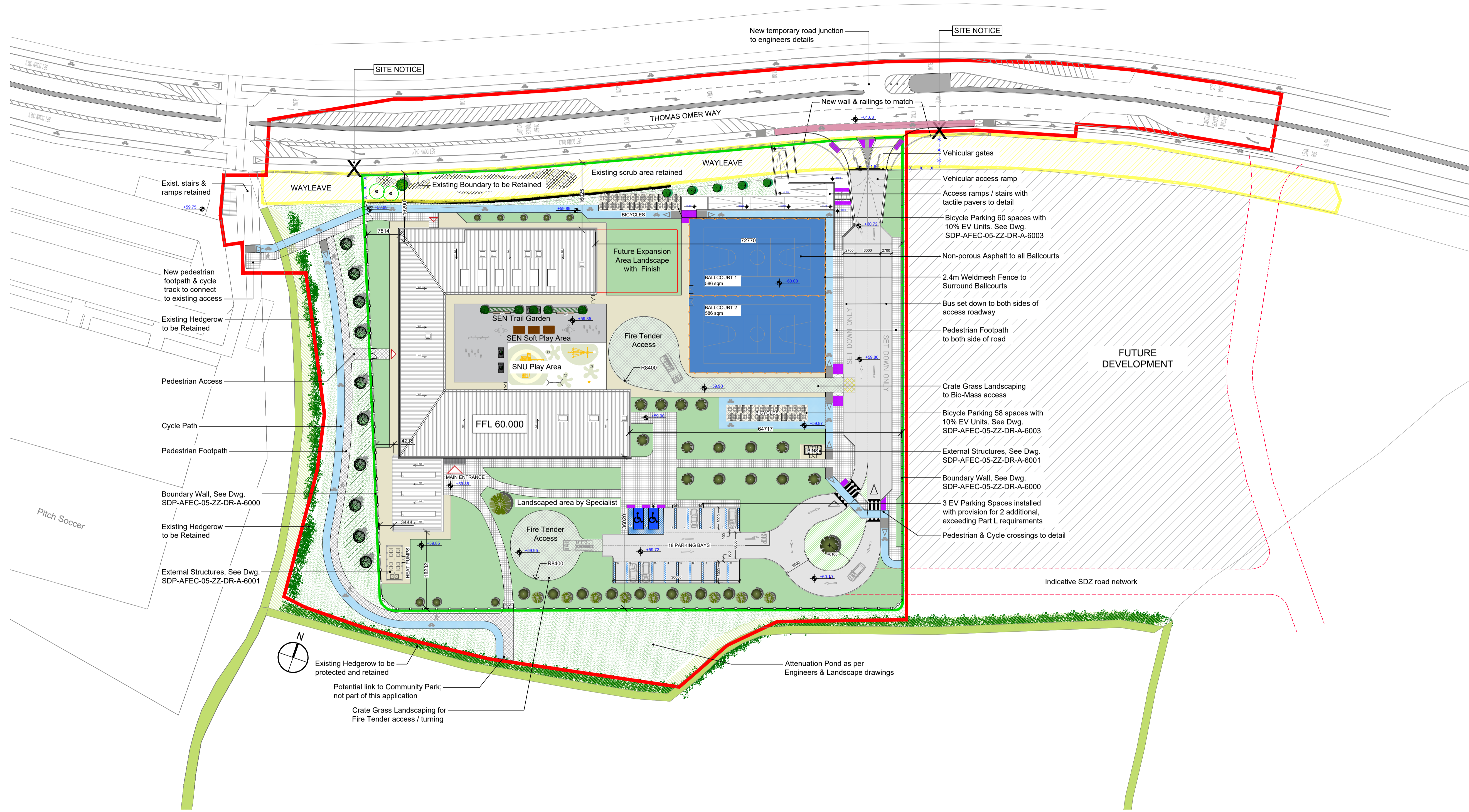
1 PROPOSED OVERALL SITE PLAN 1:500 @ A1
