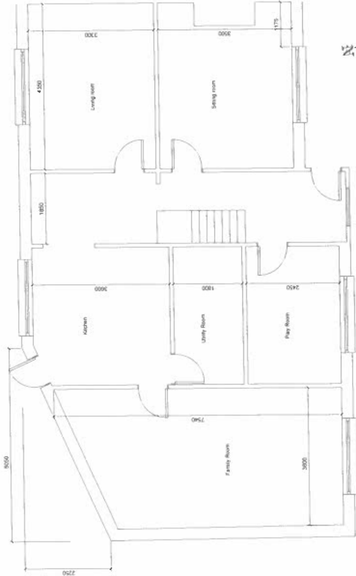
EXISTING GROUND FLOOR PLAN SCALE: 1:100 @ A4
