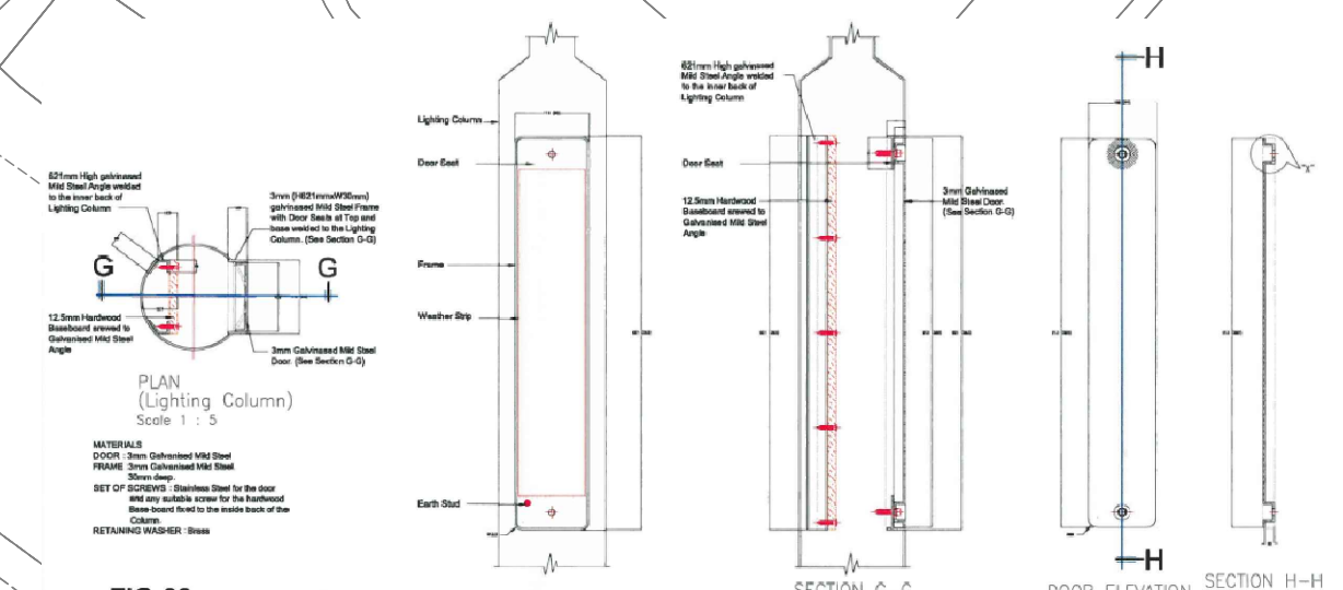
FIG-03 Lighting Column Door. SDCC FIG-03 - DETAIL DOLUMN DOOR DETAIL SPEC.
