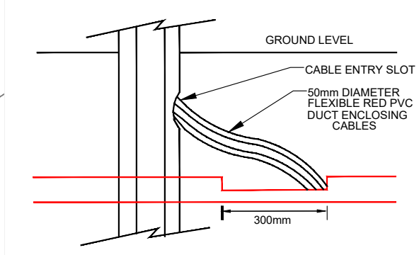
STREET LIGHT POLE - CABLING INTERFACE INSTALLATION DETAIL
