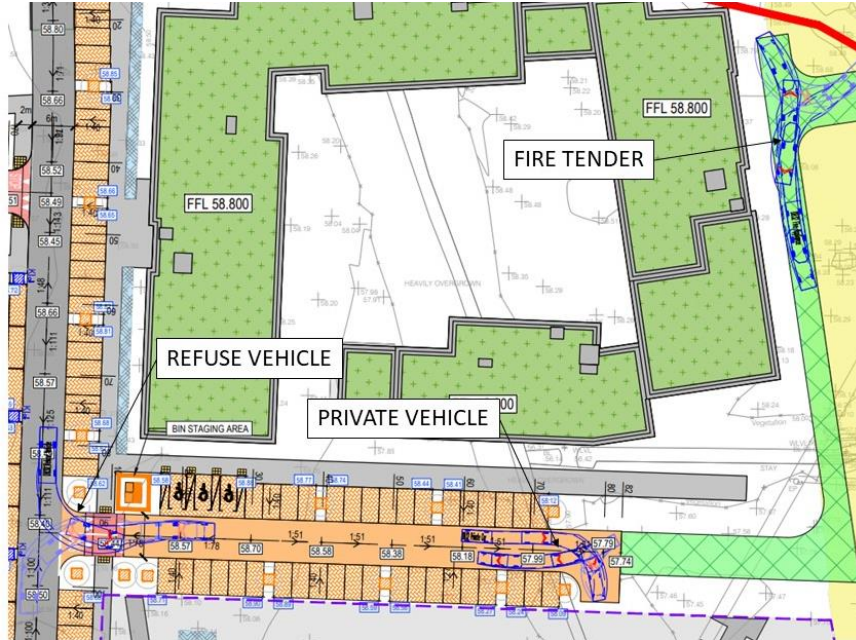
Figure 1 - Apartment Block 1 Parking Court Auto-Tracking
