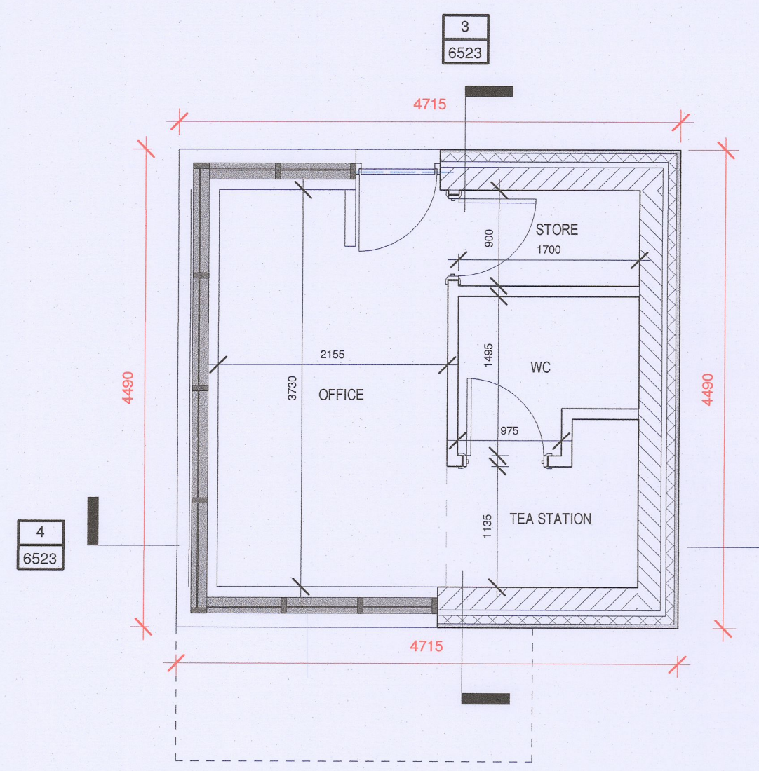
1 6523 Ground Floor Plan 1:50
