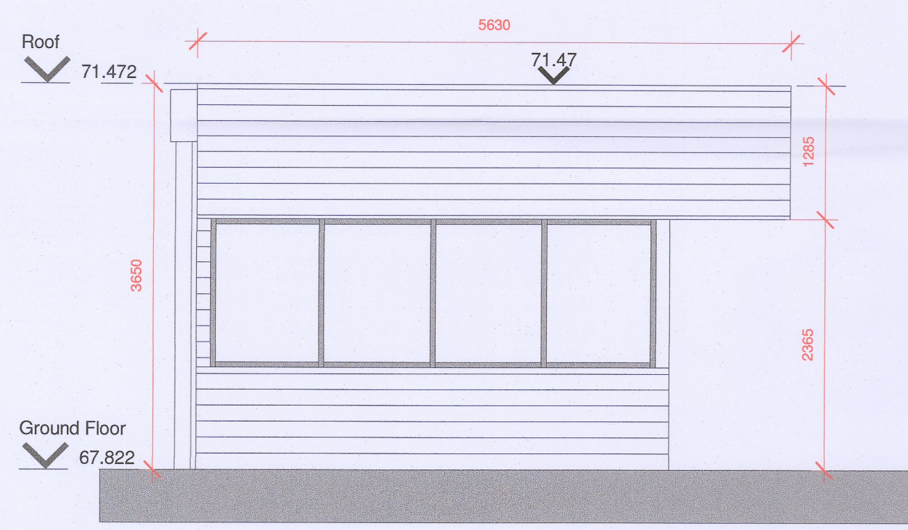
5 6523 West Elevation 1:50
