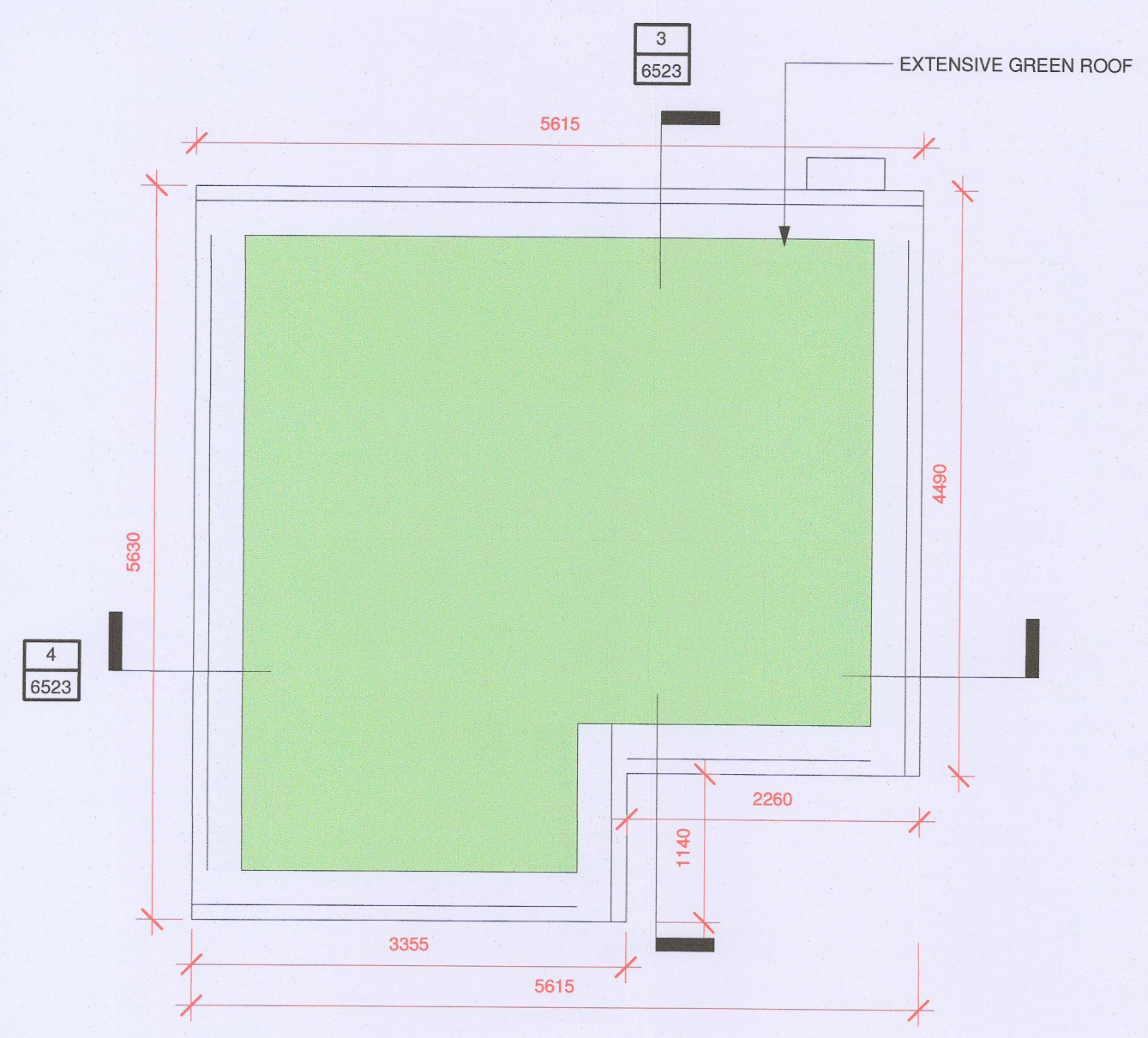
2 6523 Roof Plan 1:50
