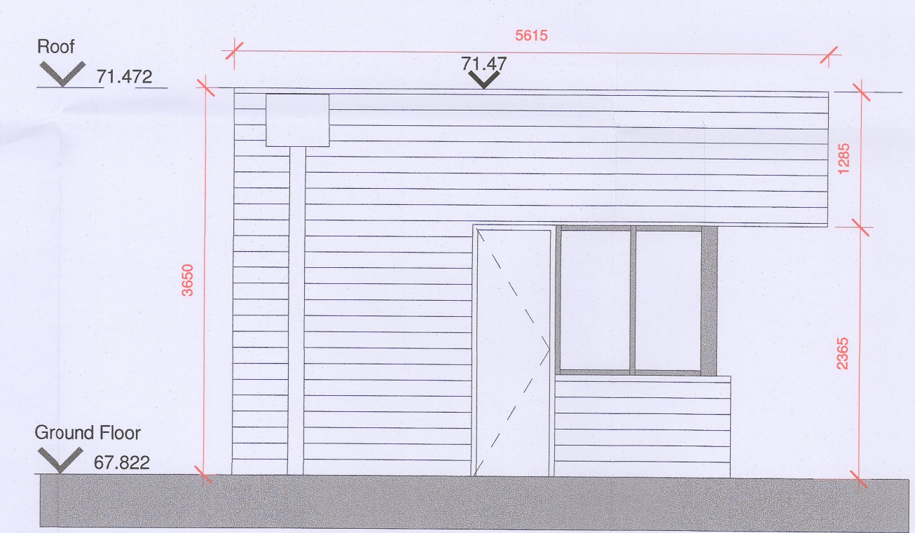
6 6523 North Elevation 1:50
