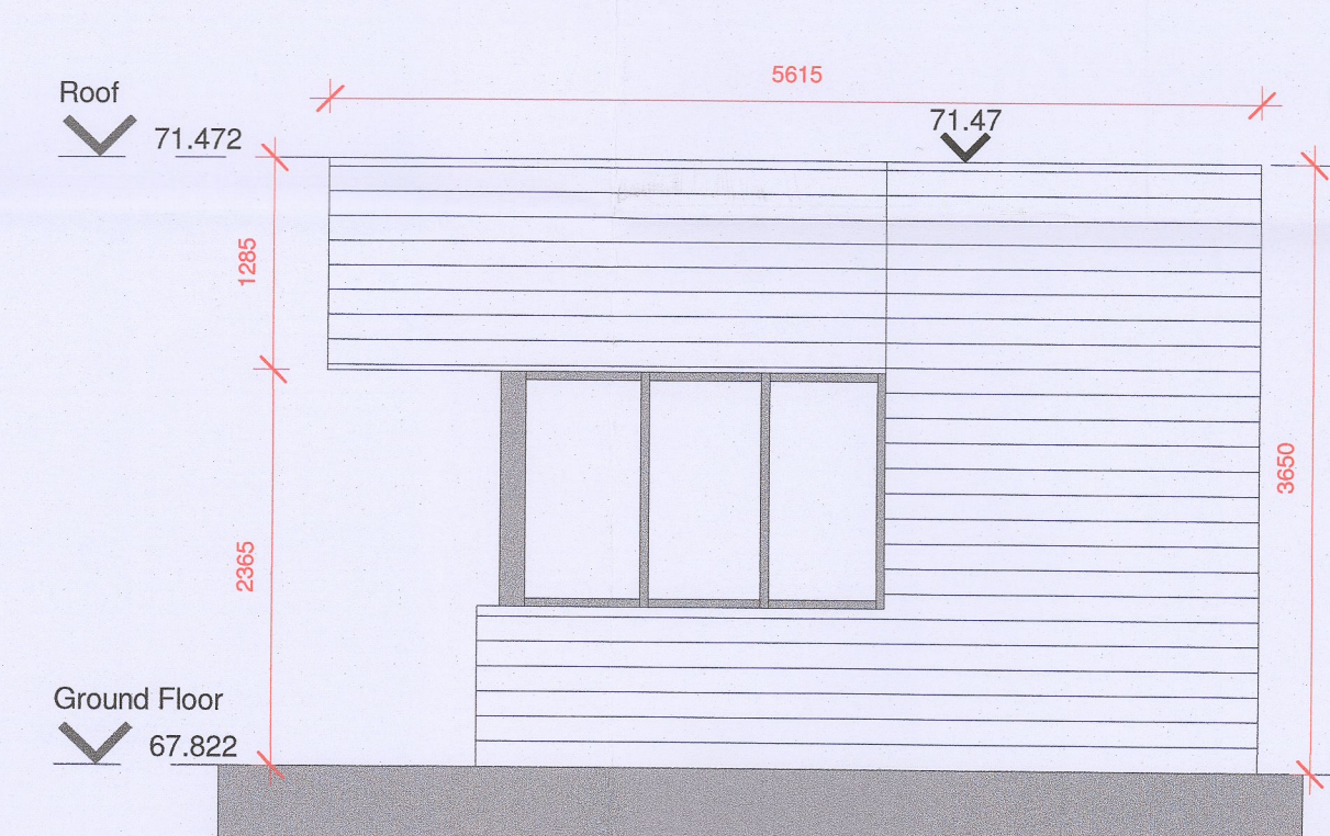
7 6523 South Elevation 1:50
