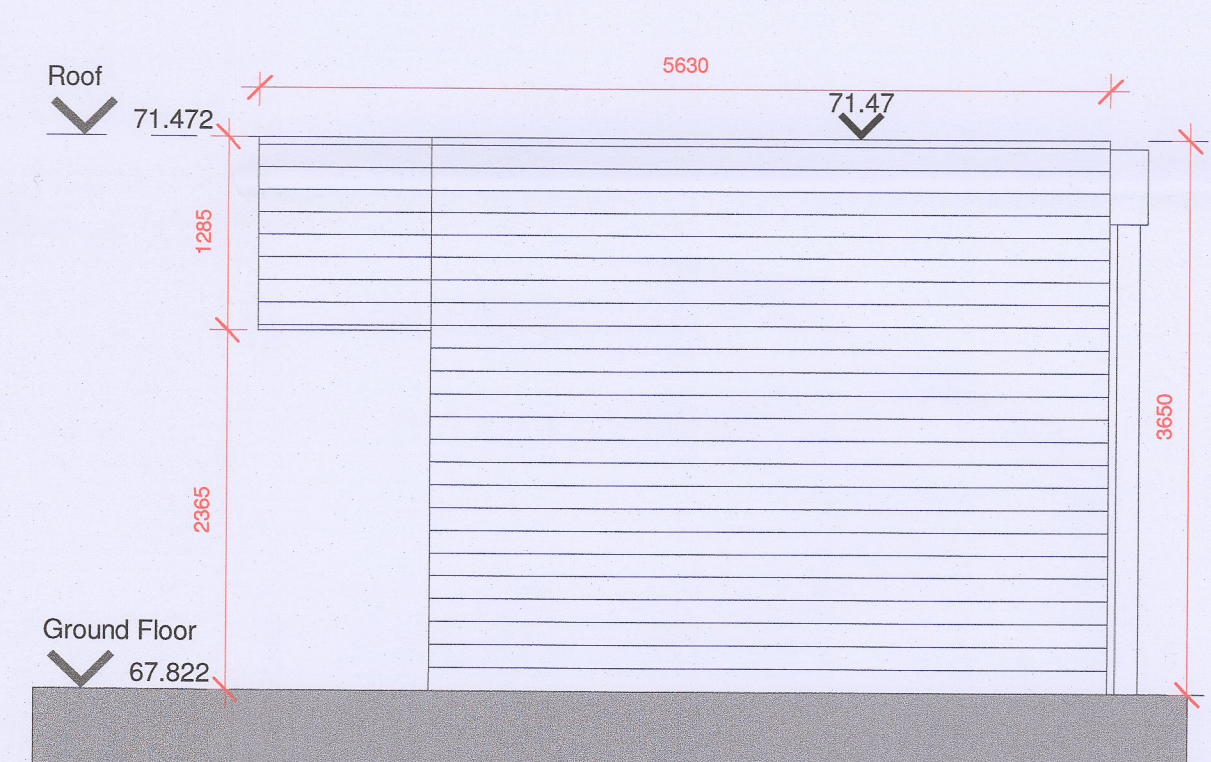
8 6523 East Elevation 1:50
