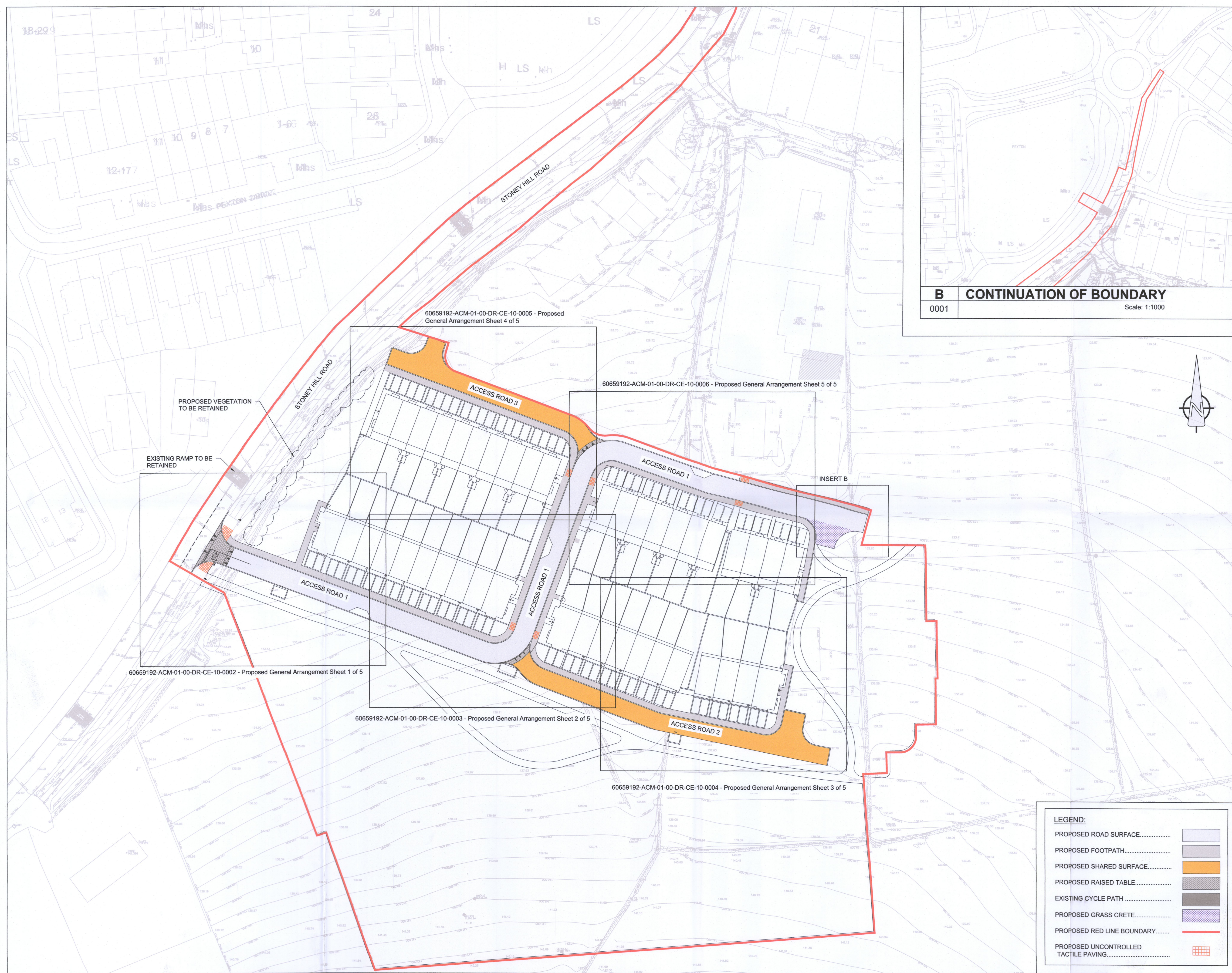
A PROPOSED GENERAL ARRANGEMENT - KEY PLAN 0001 Scale: 1:500
