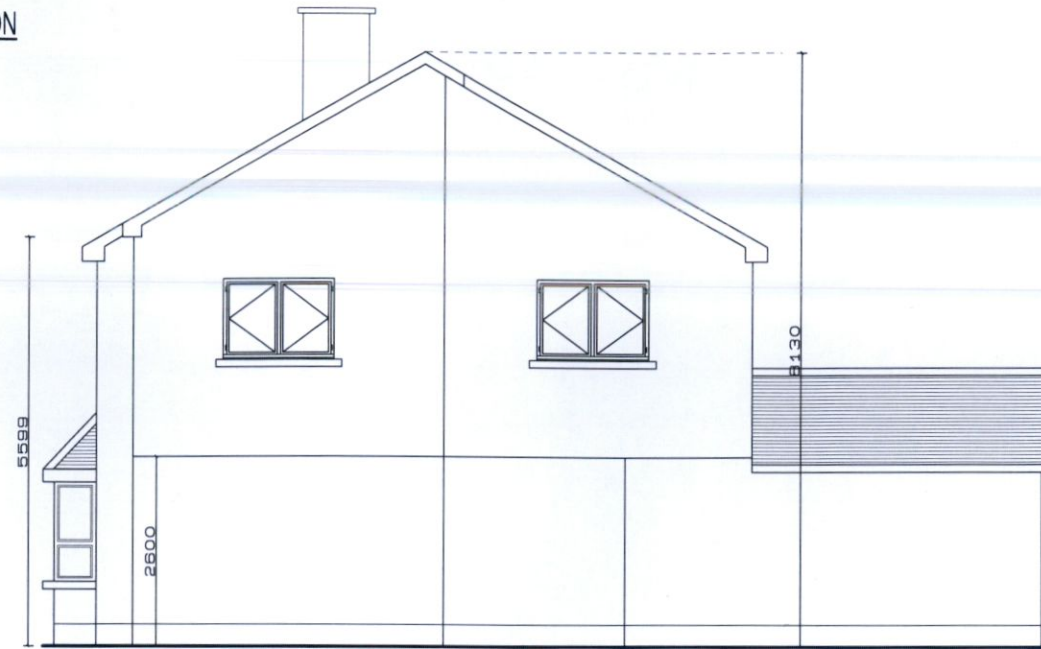
PROPOSED SIDE ELEVATION SCALE 1:100 @ A3 UPDATED
