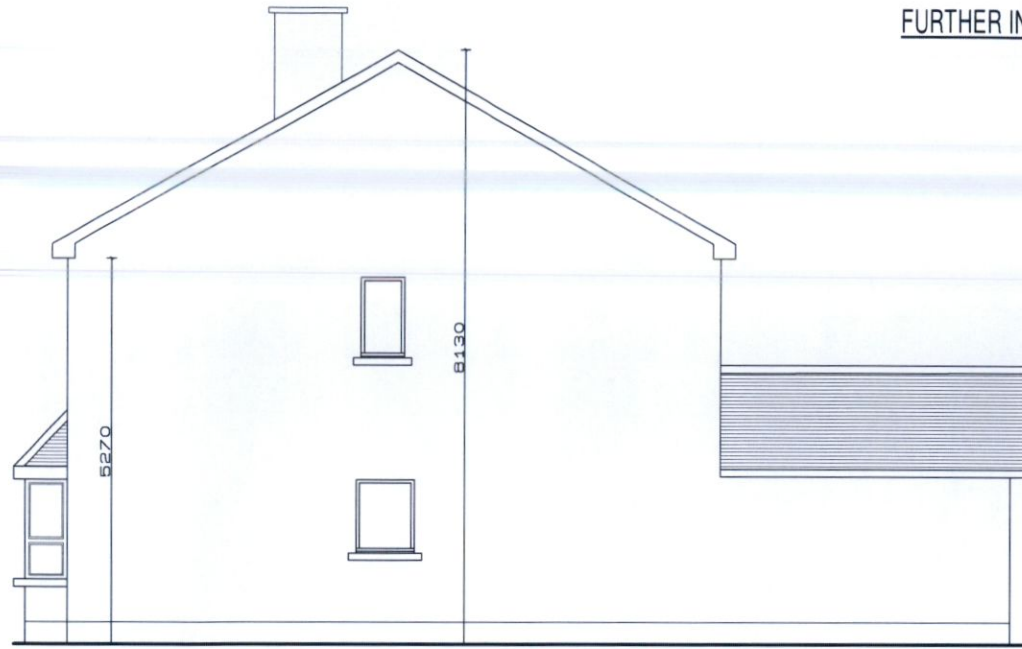
EXISTING SIDE ELEVATION SCALE 1:100 @ A3
