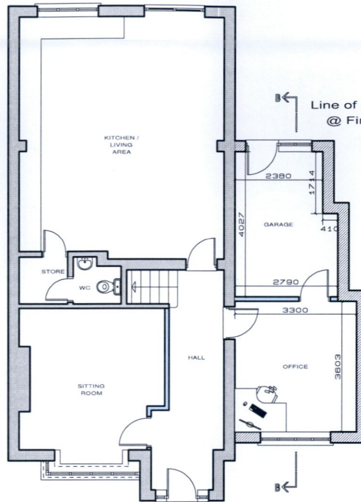
PROPOSED GROUND FLOOR PLAN SCALE 1:100 @ A3 UPDATED
