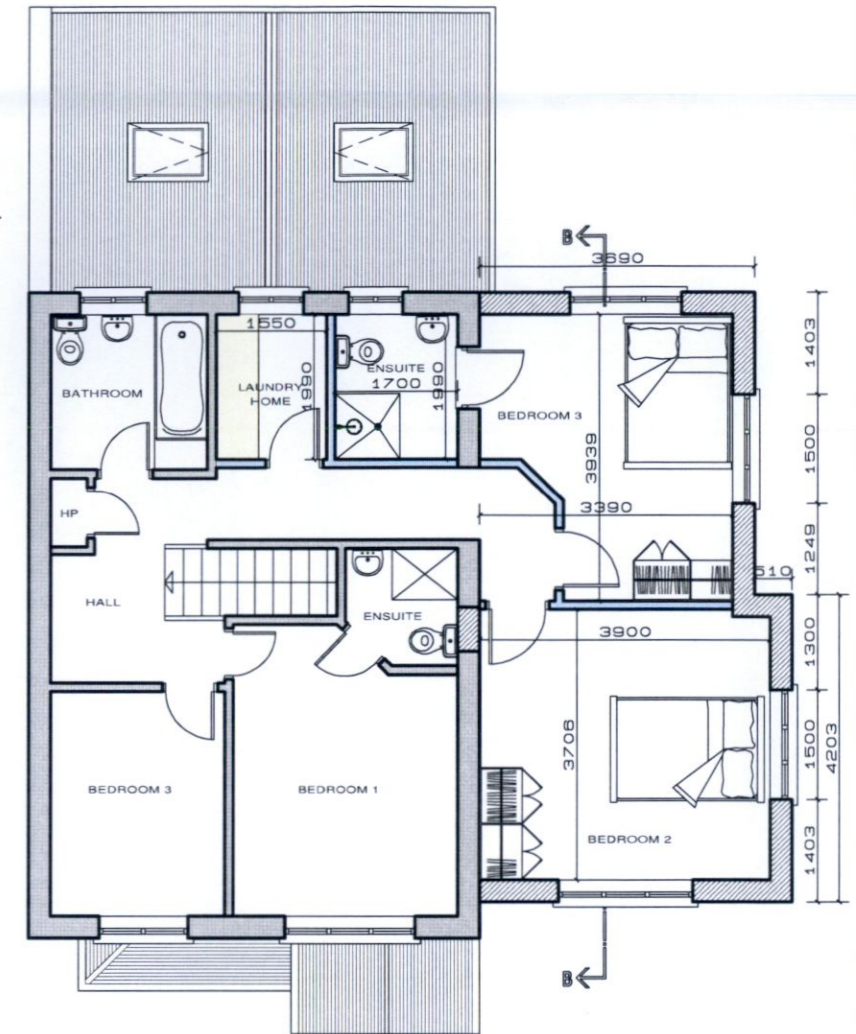
PROPOSED FIRST FLOOR PLAN SCALE 1:100 @A3 UPDATED
