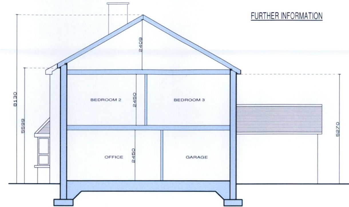
PROPOSED SECTION B-B SCALE 1:100 @ A3
