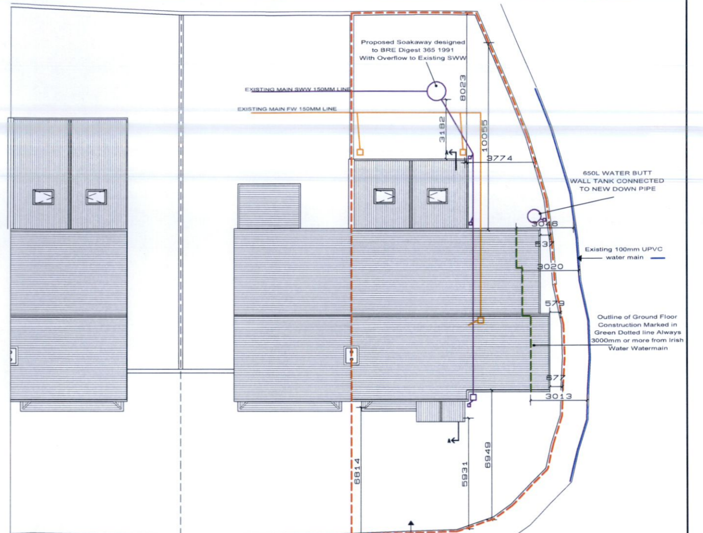
PROPOSED SITE PLAN SCALE 1:200 @A3 UPDATED
