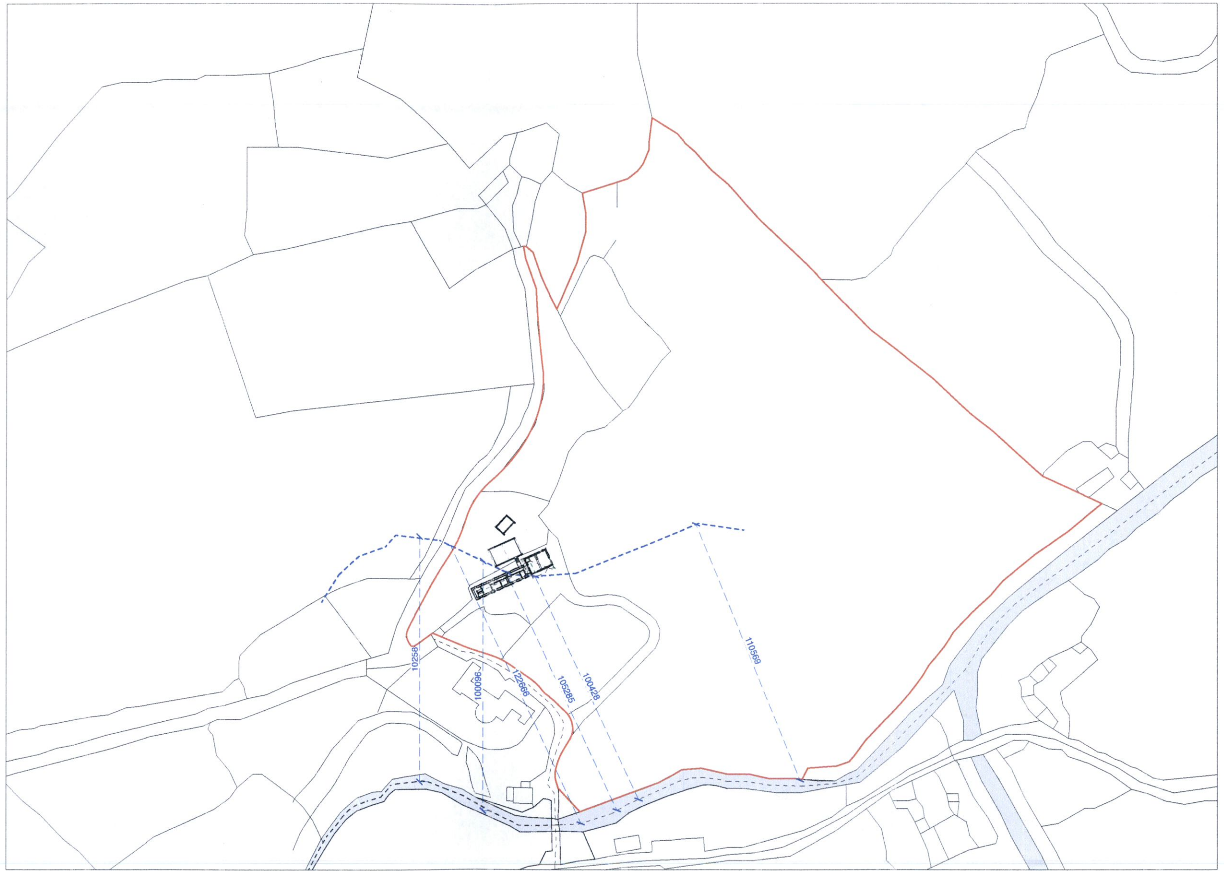
100m ZONE FROM STREAMS — SCALE 1: 1000
