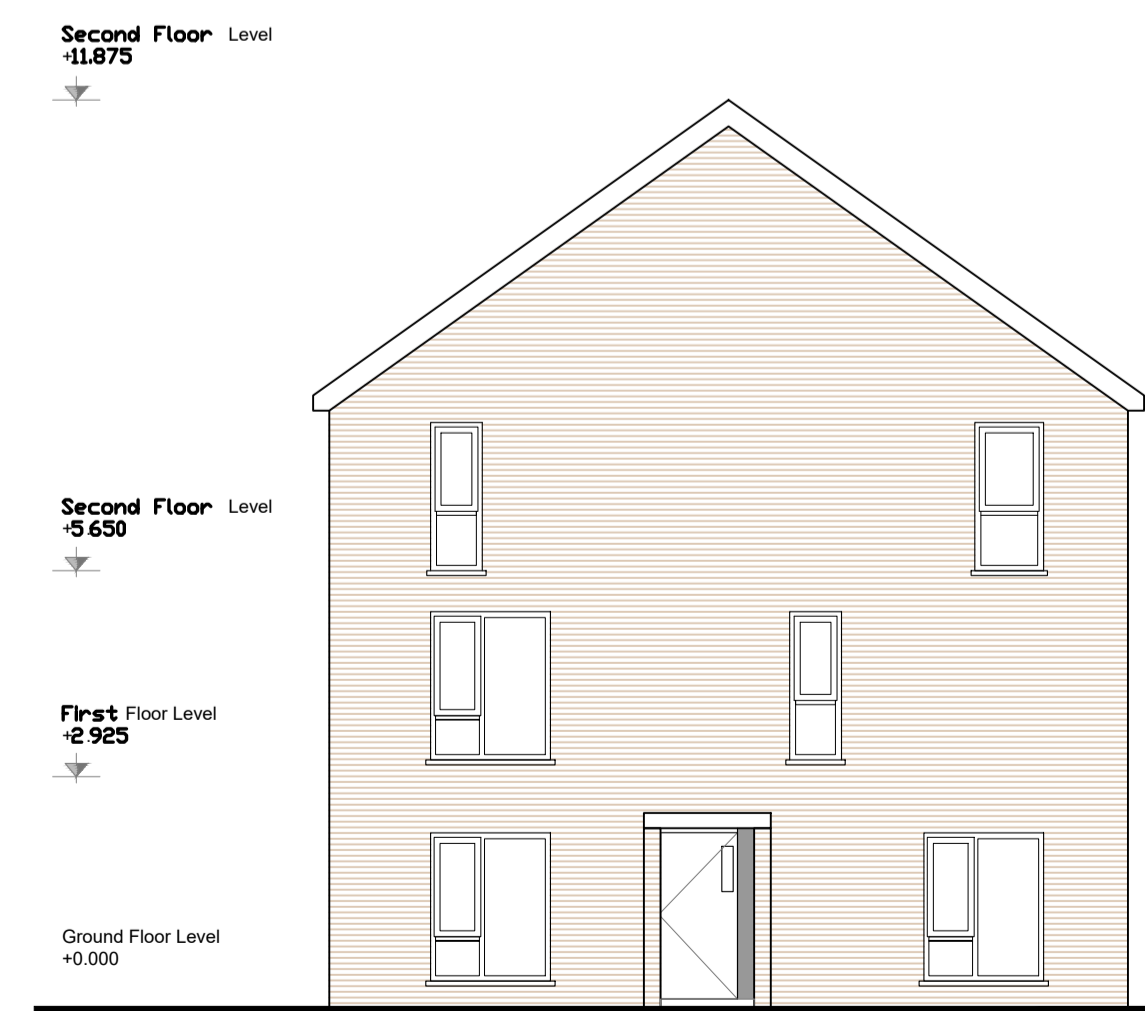
Type H4s RIGHT ELEVATION
