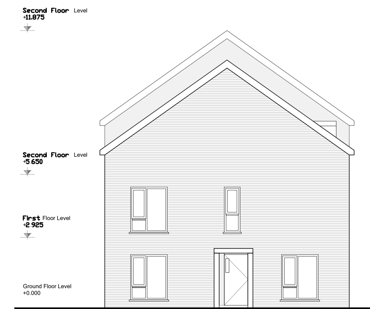
Type H3s LEFT ELEVATION
