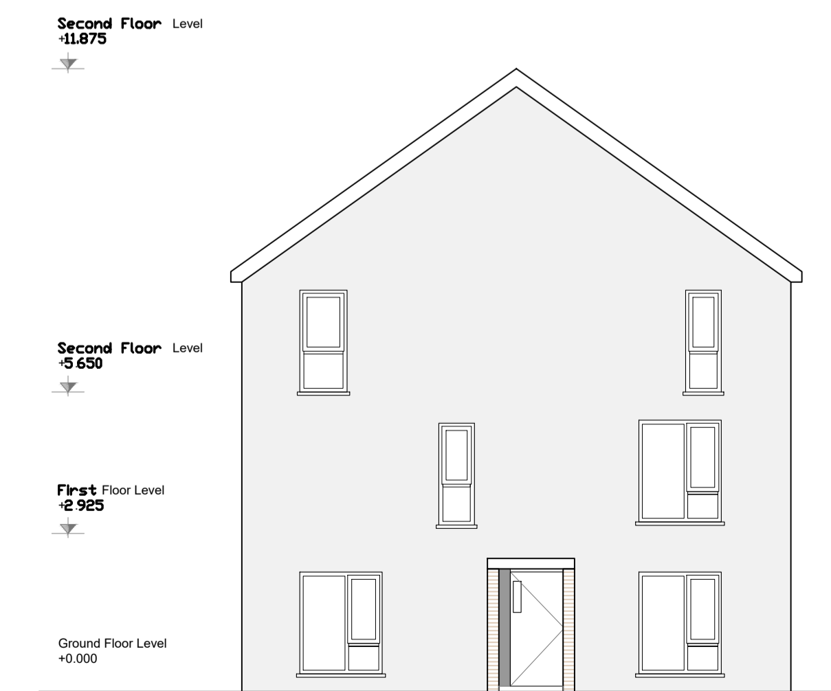
LEFT ELEVATION
