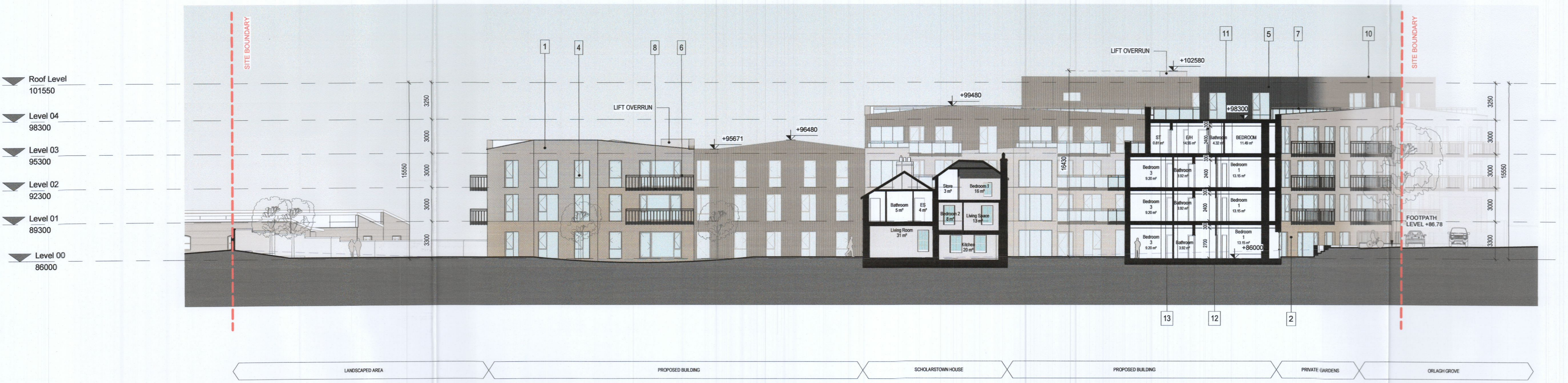
LANDSCAPED AREA PROPOSED BUILDING SCHOLARSTOWN HOUSE PROPOSED BUILDING PRIVATE GARDENS ORLAGH GROVE
