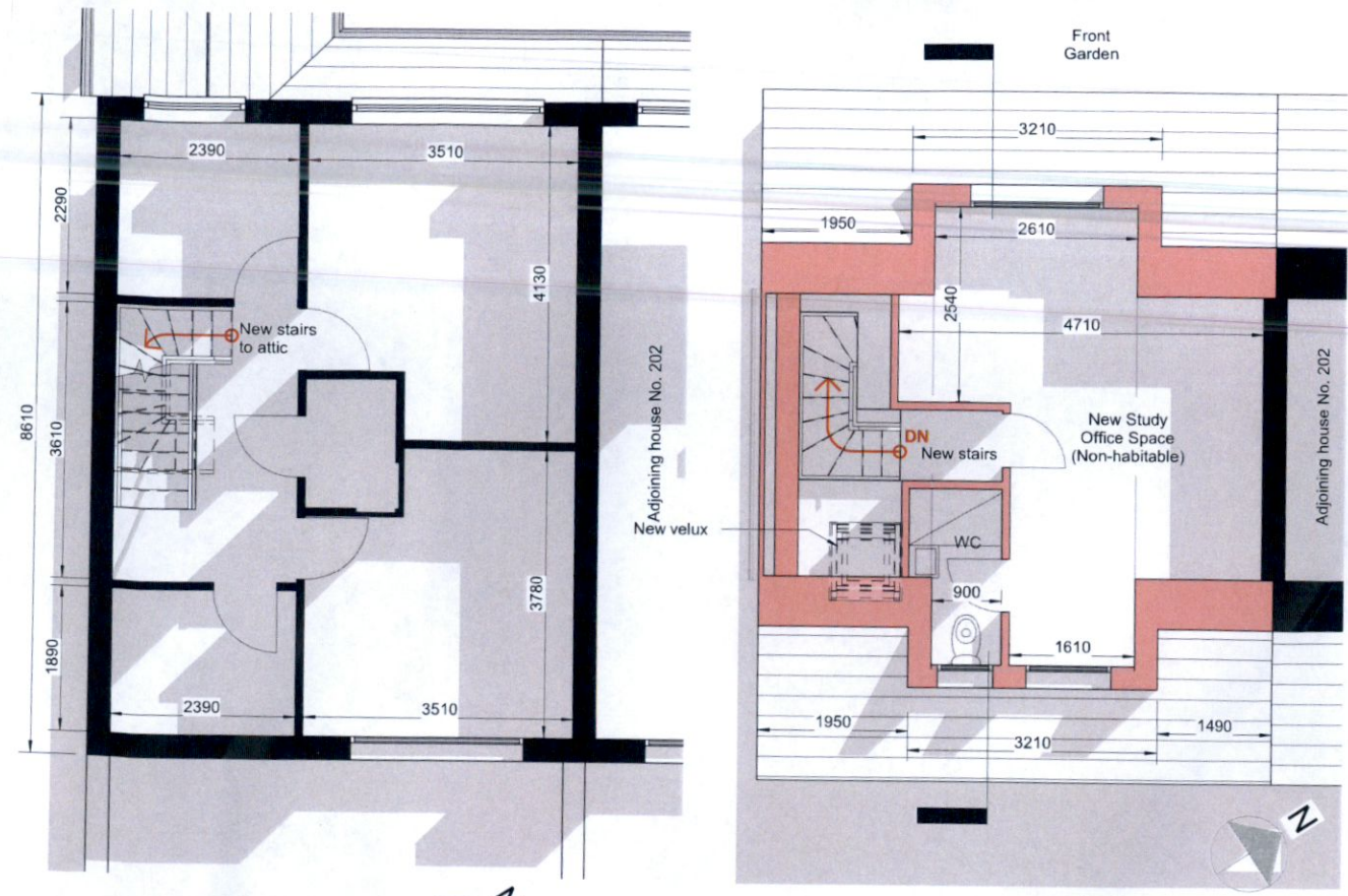
Proposed 1st Floor 1: 100
