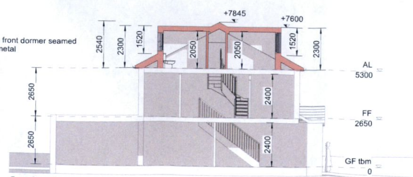
Section 1 1: 200
