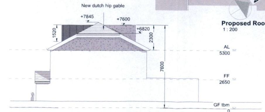
Proposed South-Side Elevation 1: 200
