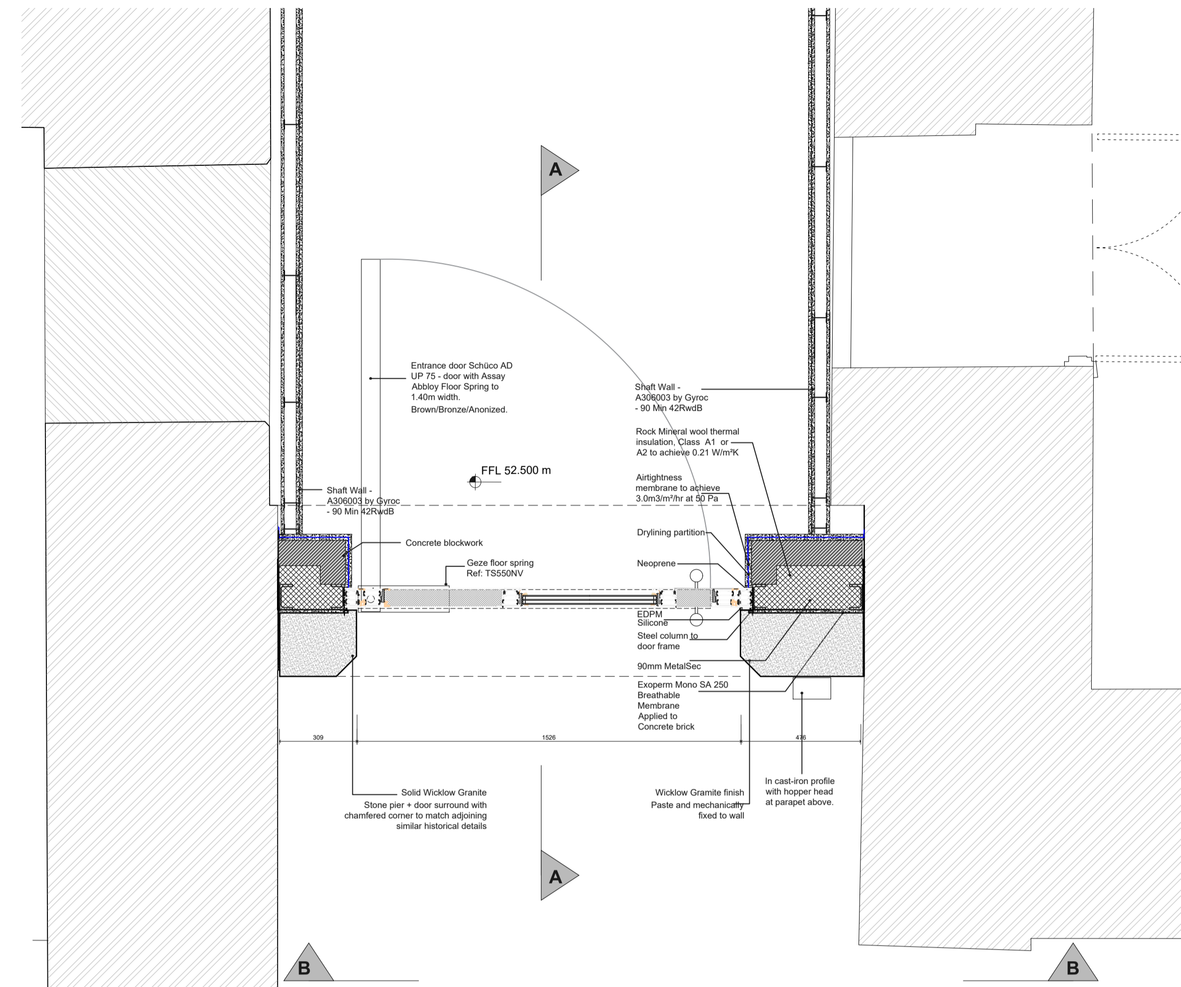
Plan GORUND FLOOR - DET 2- 1:15
