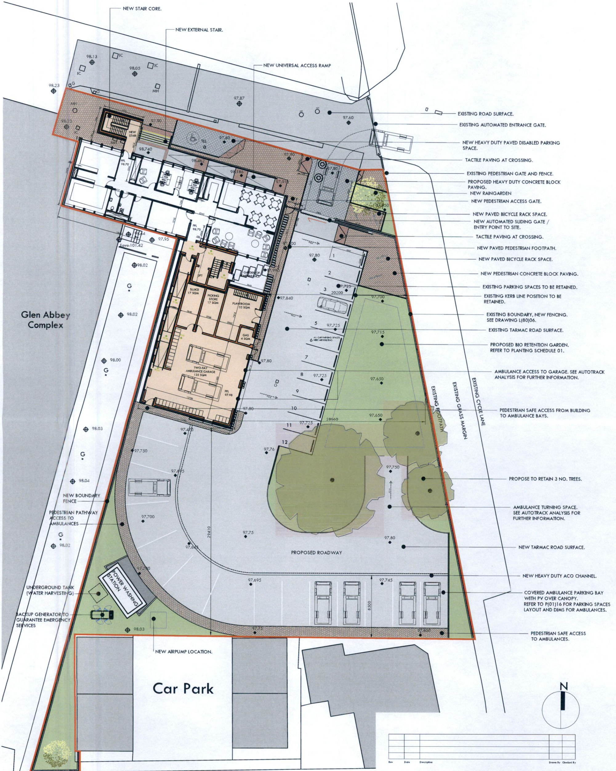
PROPOSED LANDSCAPE PLAN Scale 1:300
