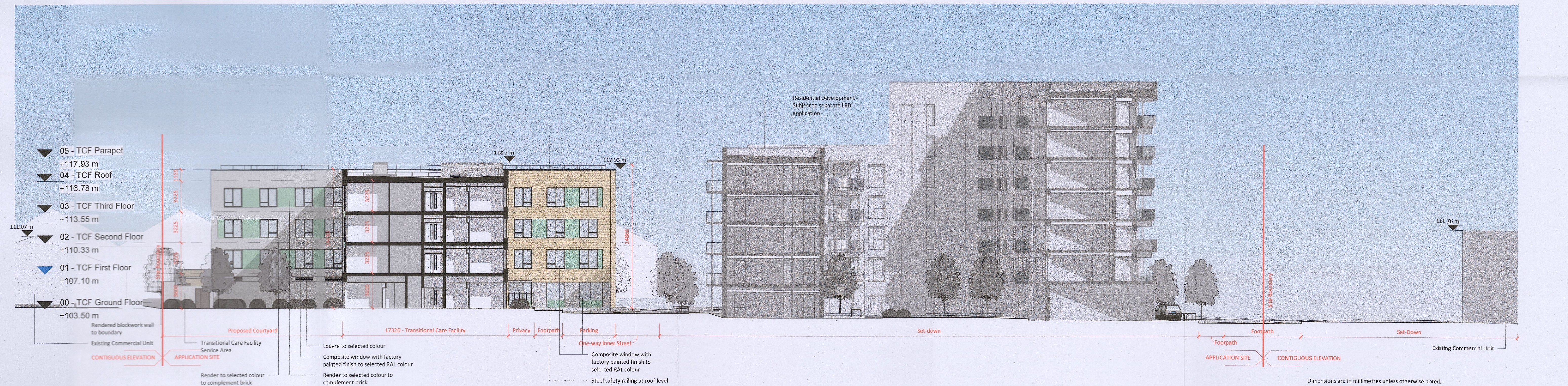
2 Proposed Section D-D - Transitional Care Facility 1:200
