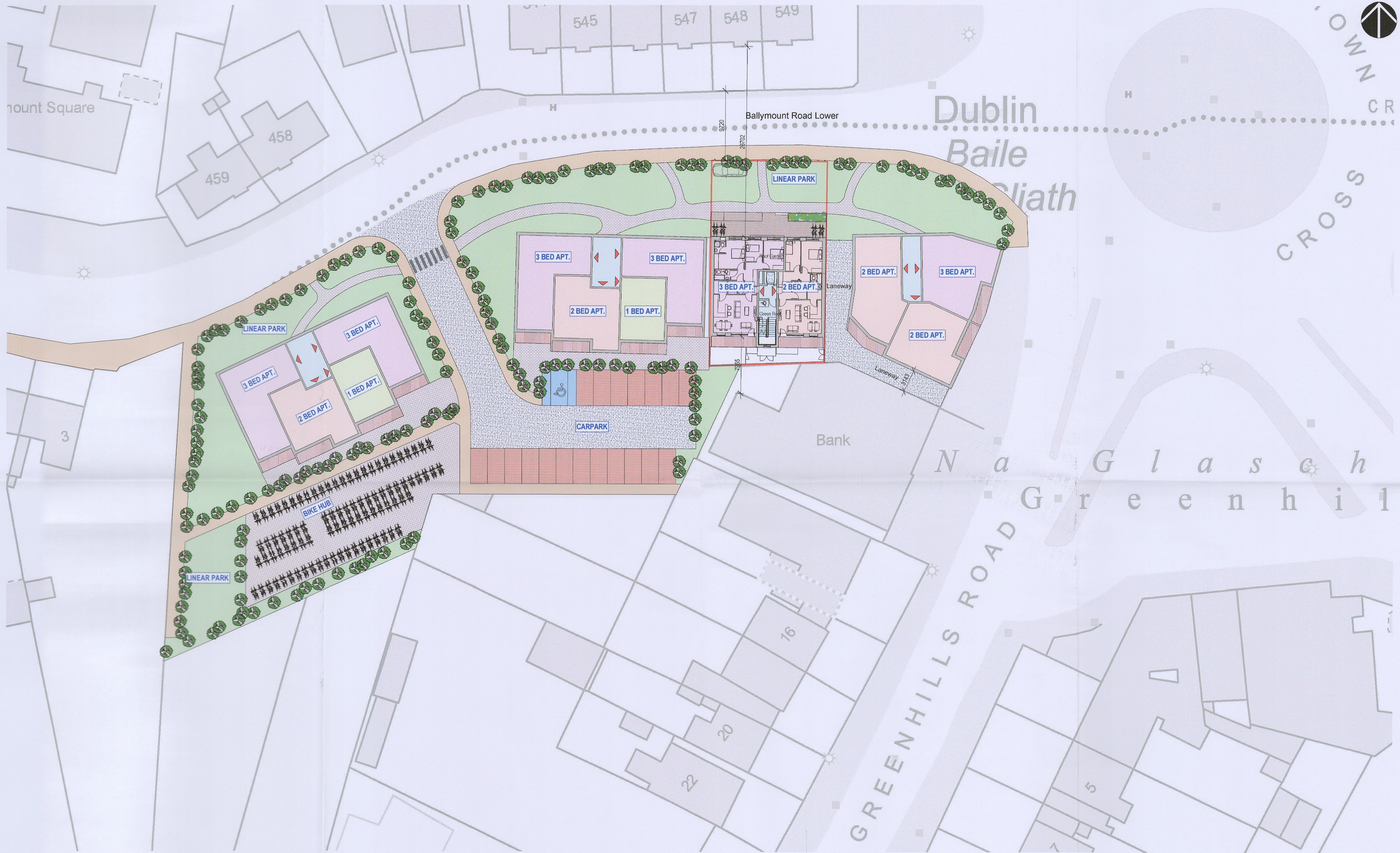
1 PROPOSED MASTERPLAN SCALE 1: 250
