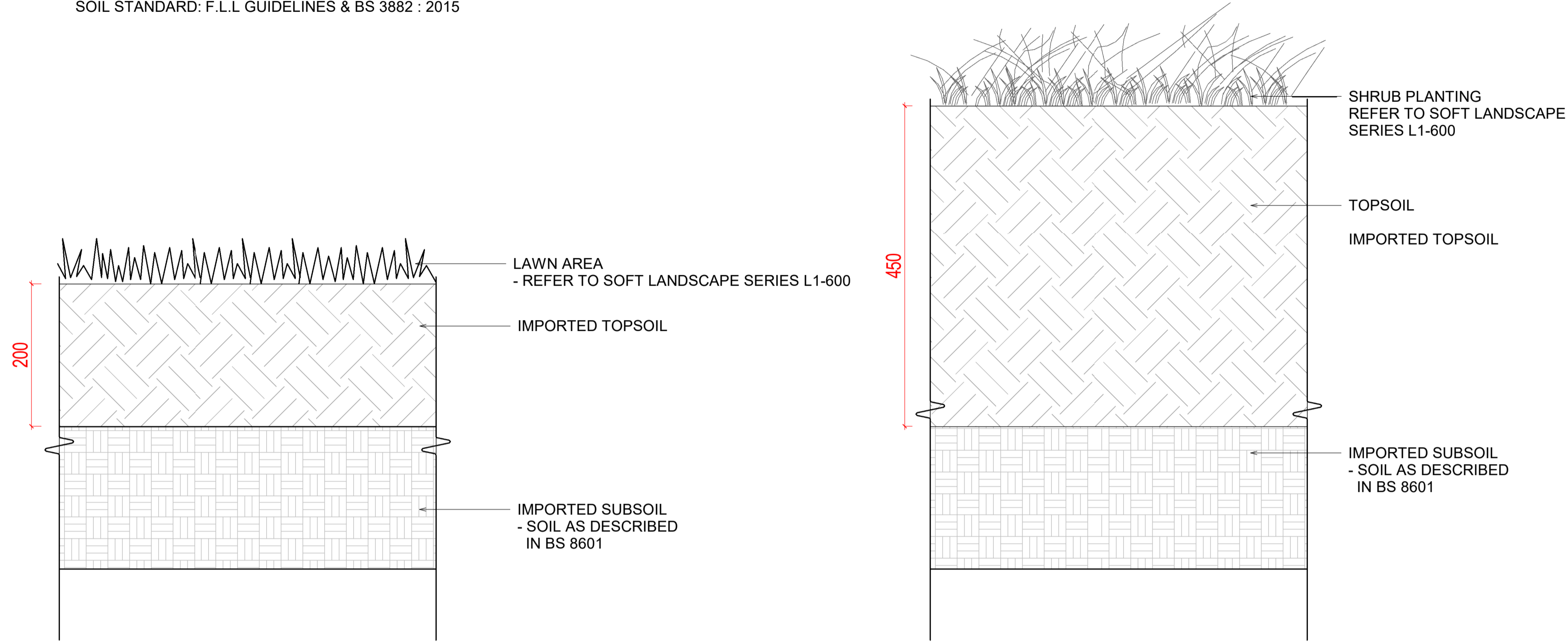
TURF SOIL PROFILE TO NATURAL GROUND AREAS
