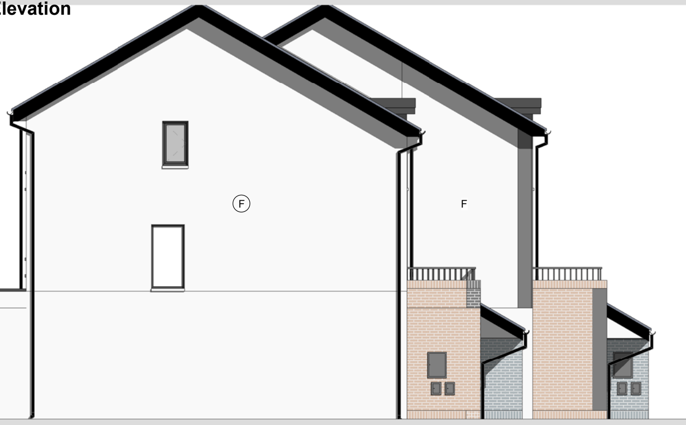
Existing Side Elevation 1
