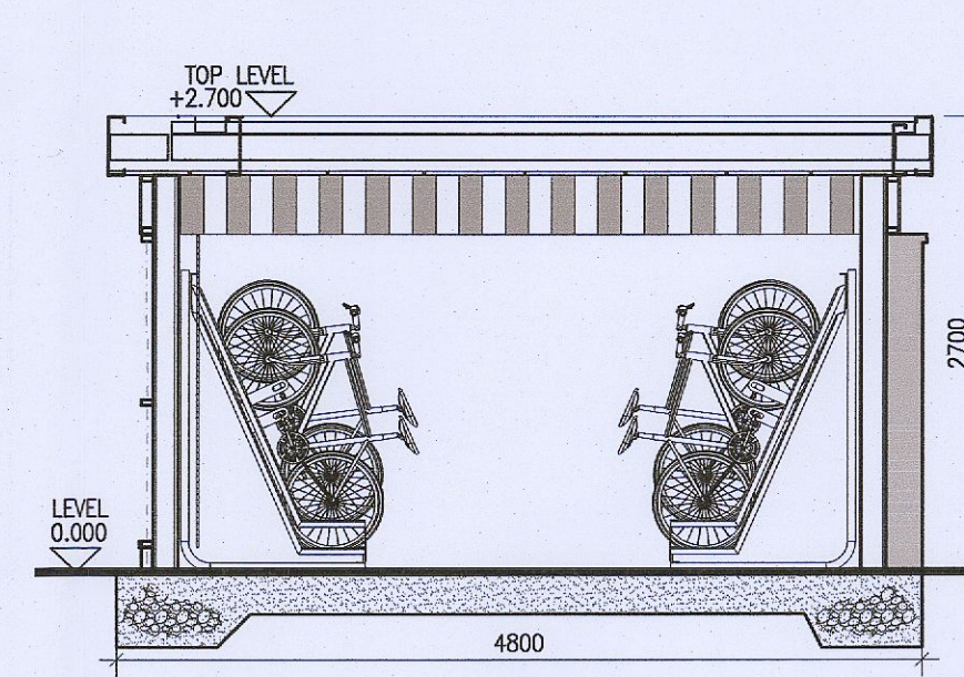
7 Bike Store Type 3 Section AA Scale 1:50
