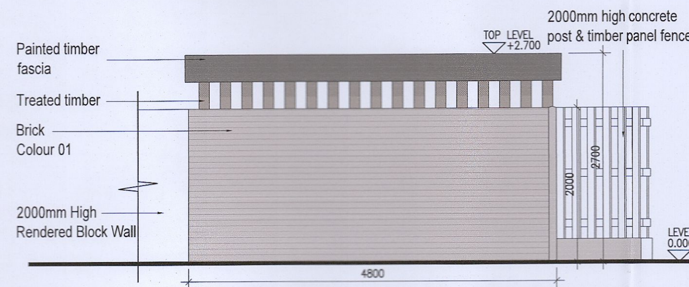
4 Bike Store Type 3 Side Elevation 01 Scale 1:50
