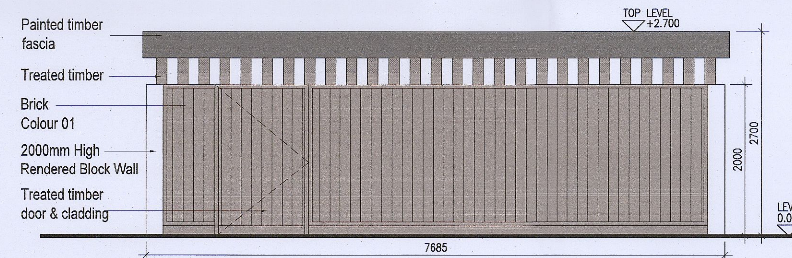
5 Bike Store Type 3 Front Elevation Scale 1:50
