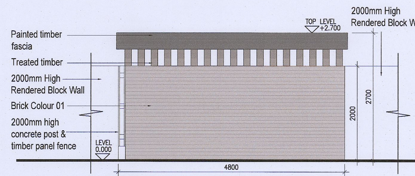
6 Bike Store Type 3 Side Elevation 02 Scale 1:50
