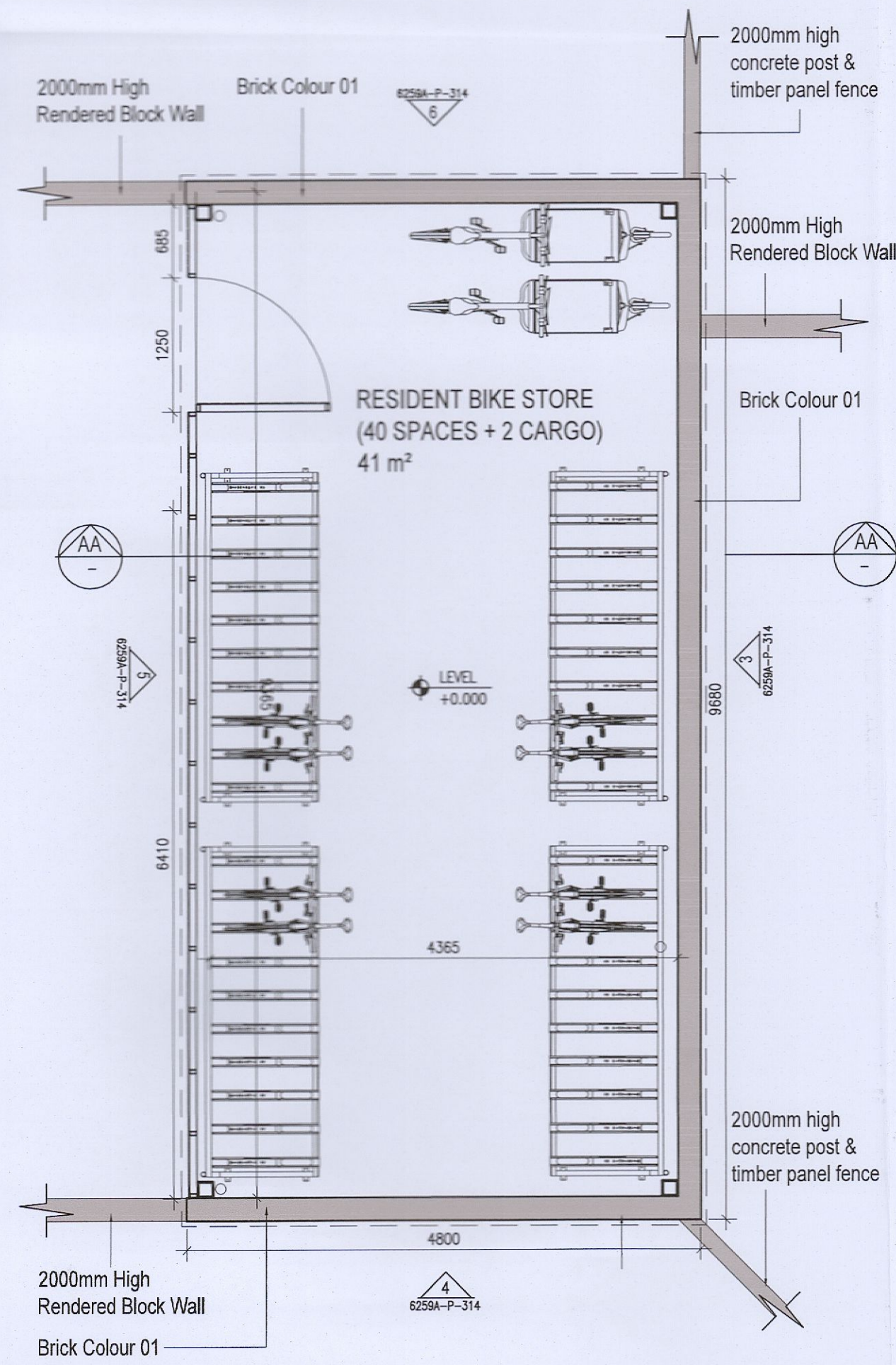
1 Bike Store Type 3 Plan Scale 1:50
