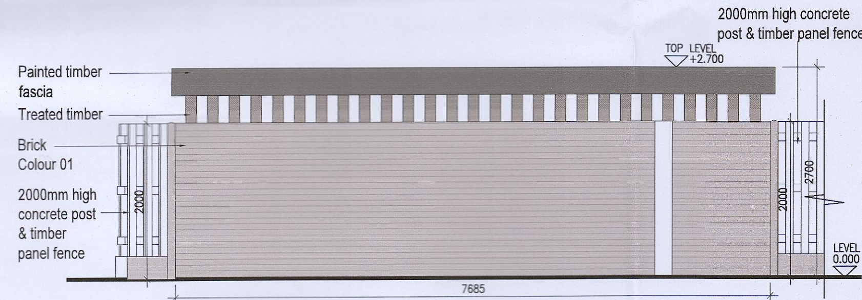
3 Bike Store Type 3 Rear Elevation Scale 1:50
