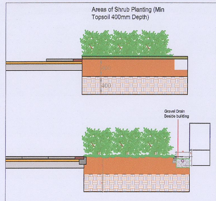
Typical Landscape details of soil Depth Scale (1:50 @A1)
