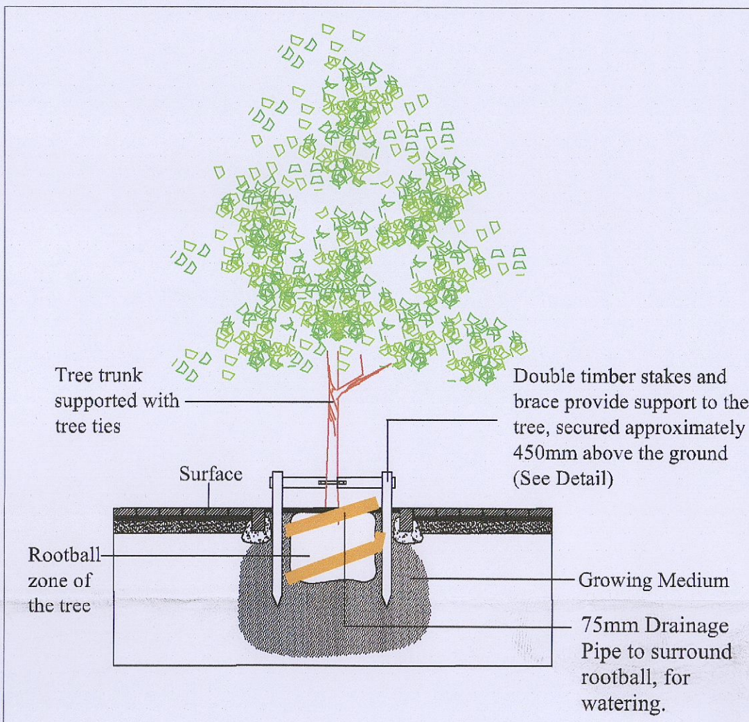
Typical Tree Stake Detail Scale (1:50 @A1)
