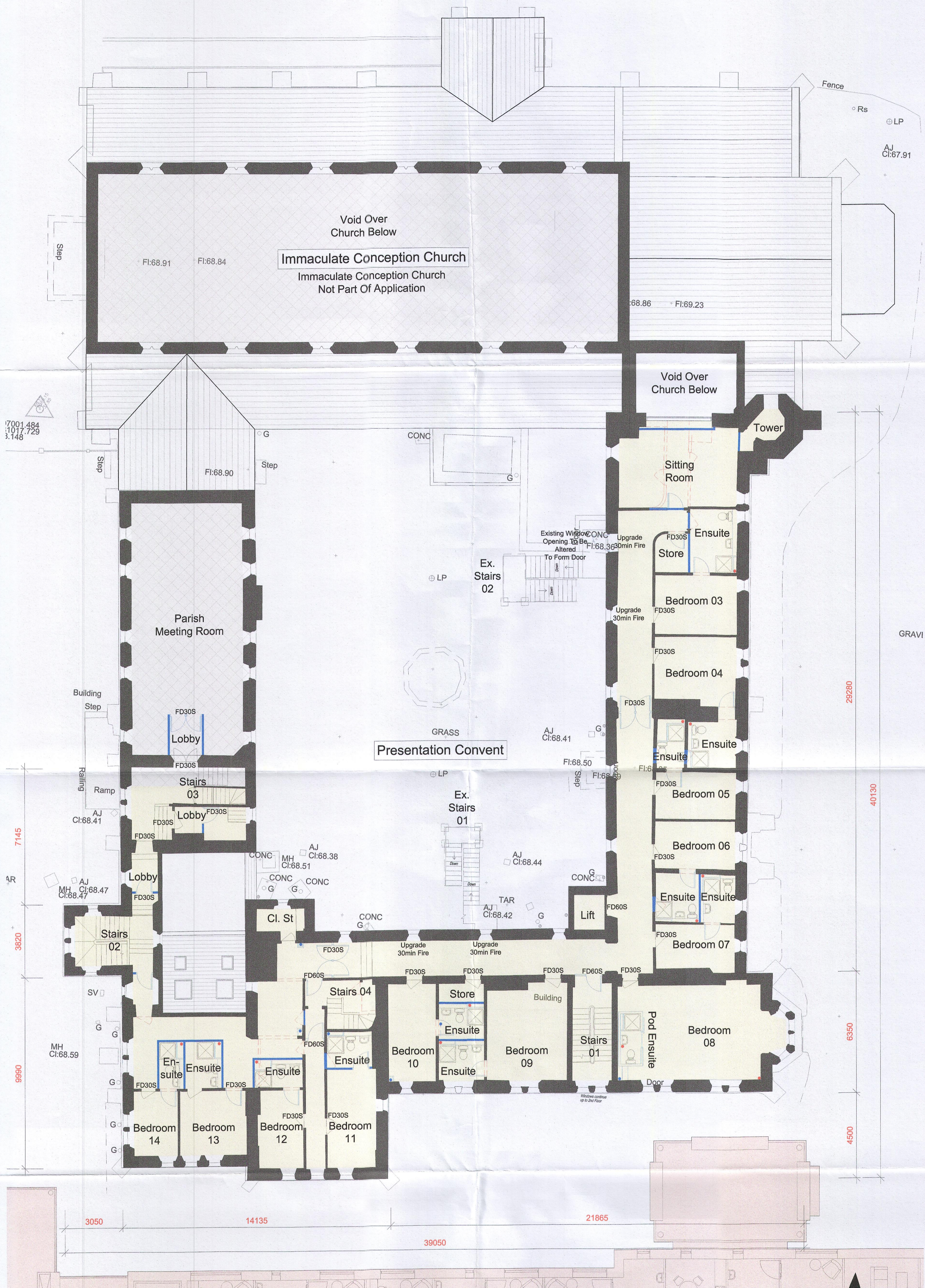
PROPOSED FIRST FLOOR PLAN
