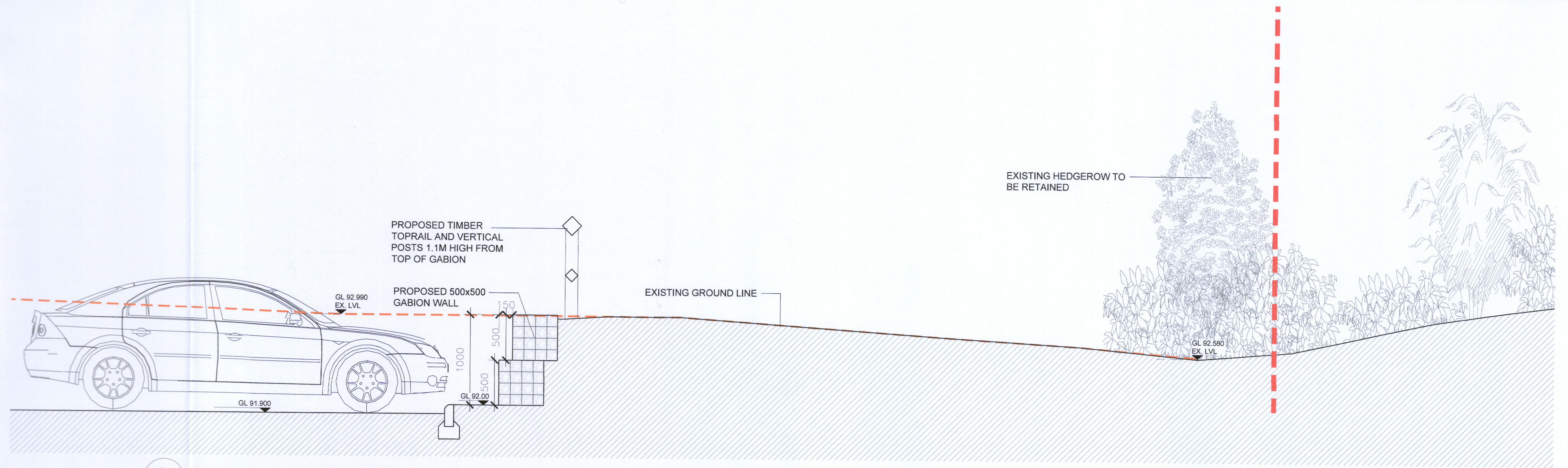
01 Proposed Boundary Treatment (Boundaries D-E) Section PA 503 1:25
