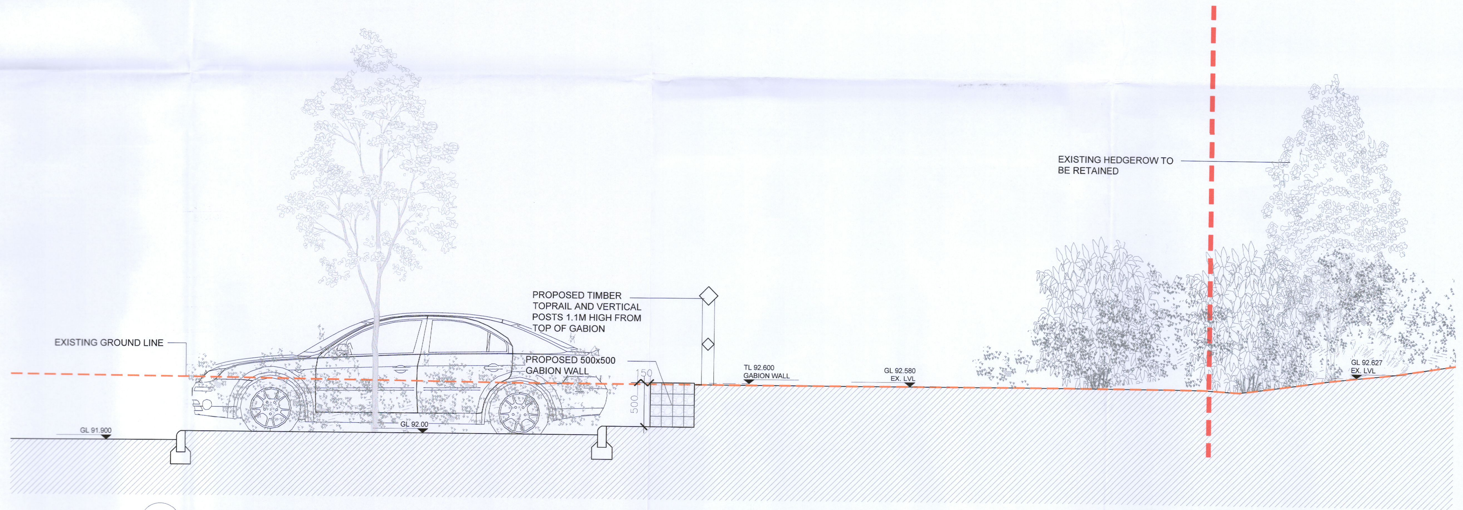
02 Proposed Boundary Treatment (Boundaries D-E) Section PA 503 1:25
