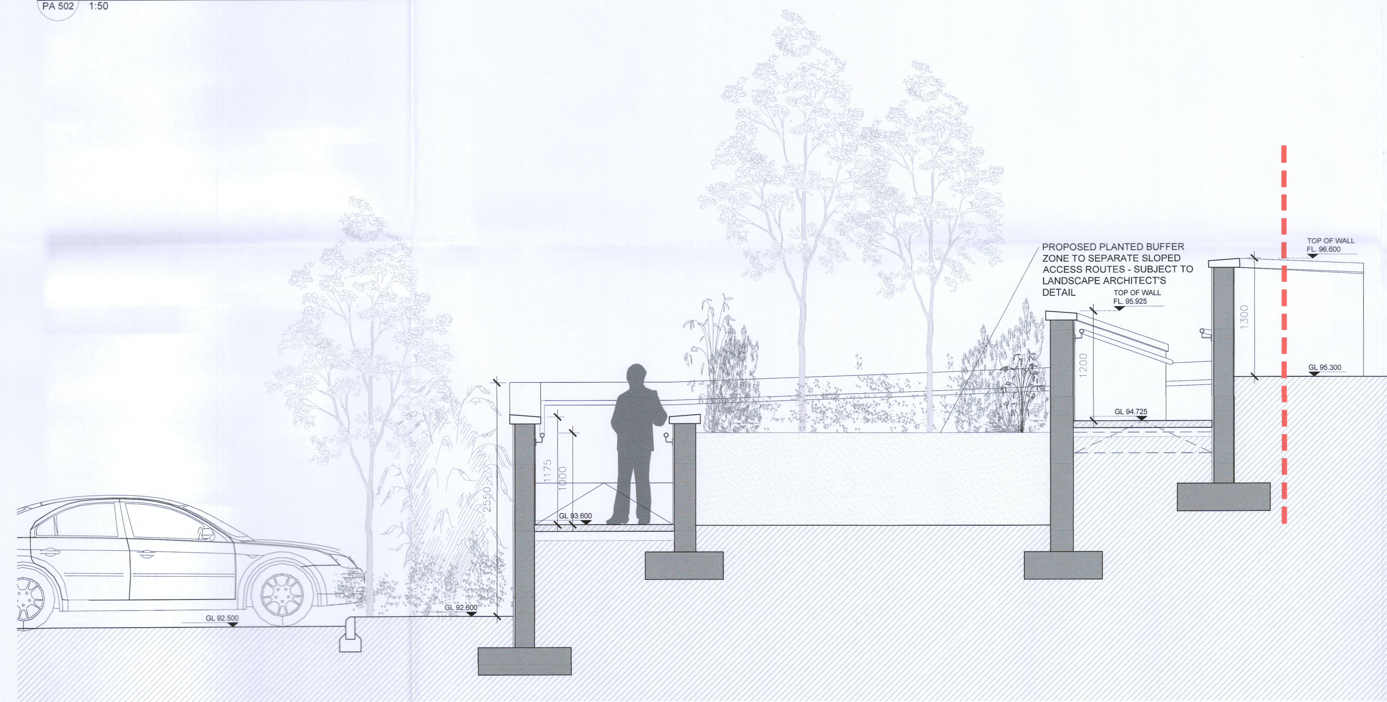
02 Proposed Boundary Treatment (Boundaries I-J) Section PA 502 1:25
