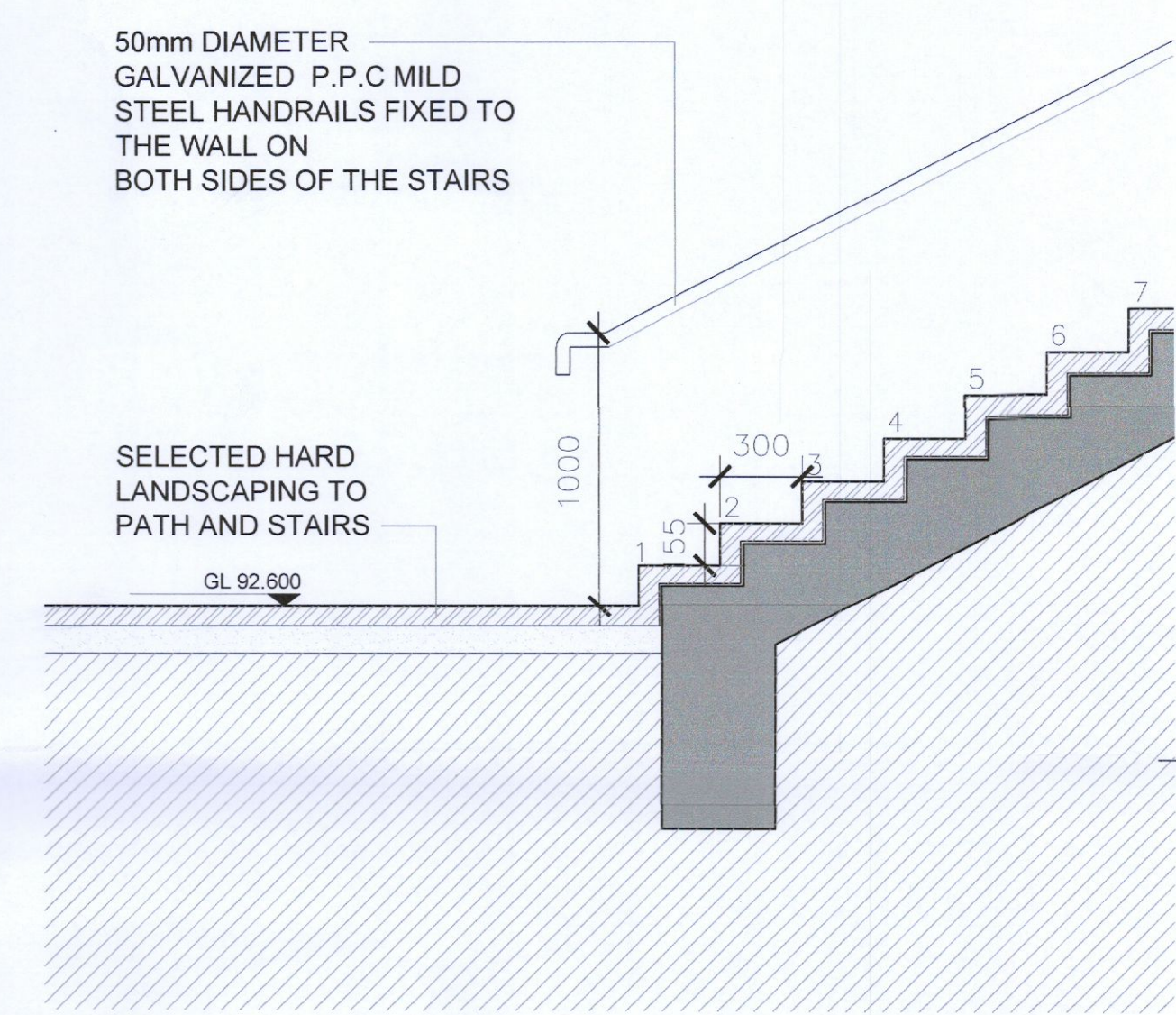
03 Proposed Stairs Section (Boundaries I-J) PA 502 1:25
