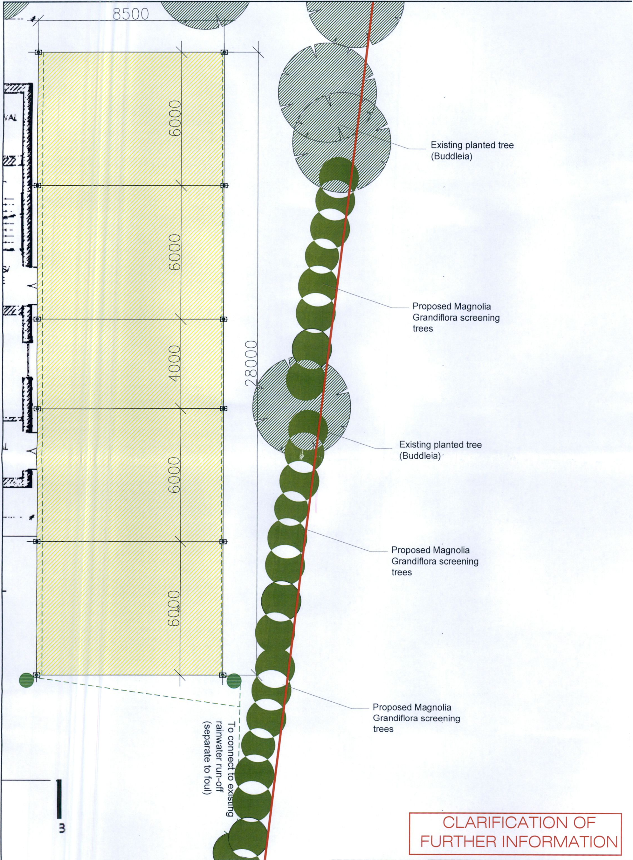
Landscaping Plan
