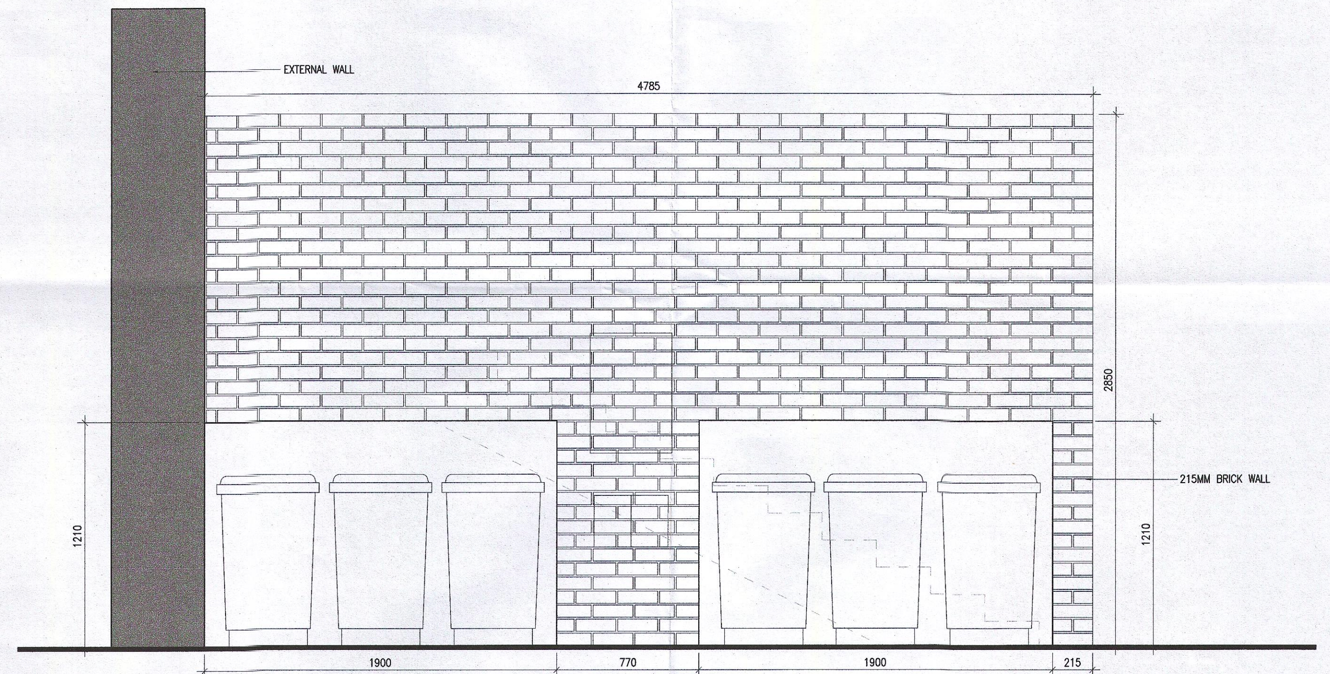
3 Bin store Type 4 Side Elevation 704 Scale 1:20
