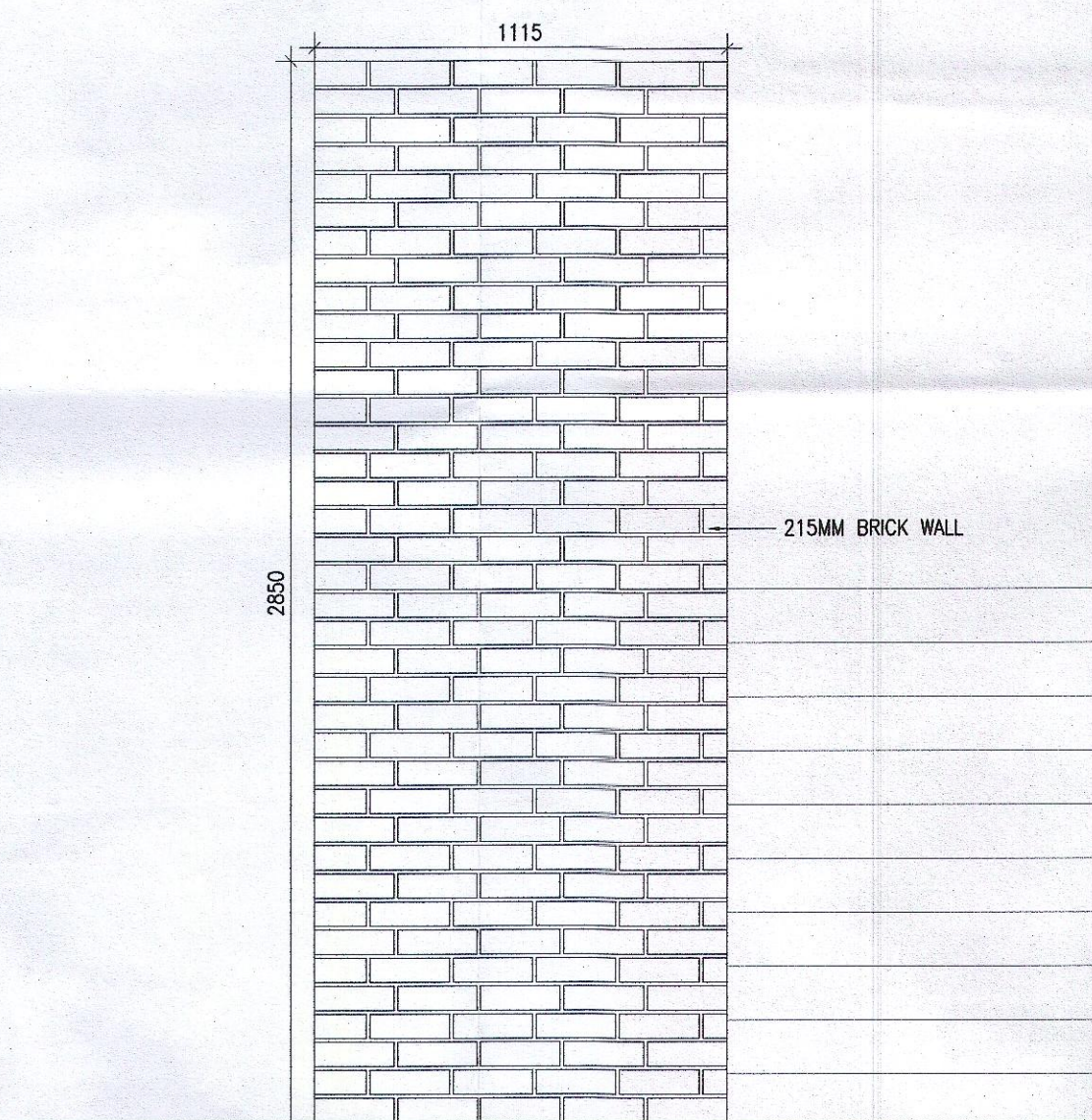
2 Bin store Type 4 Front Elevation 704 Scale 1:20
