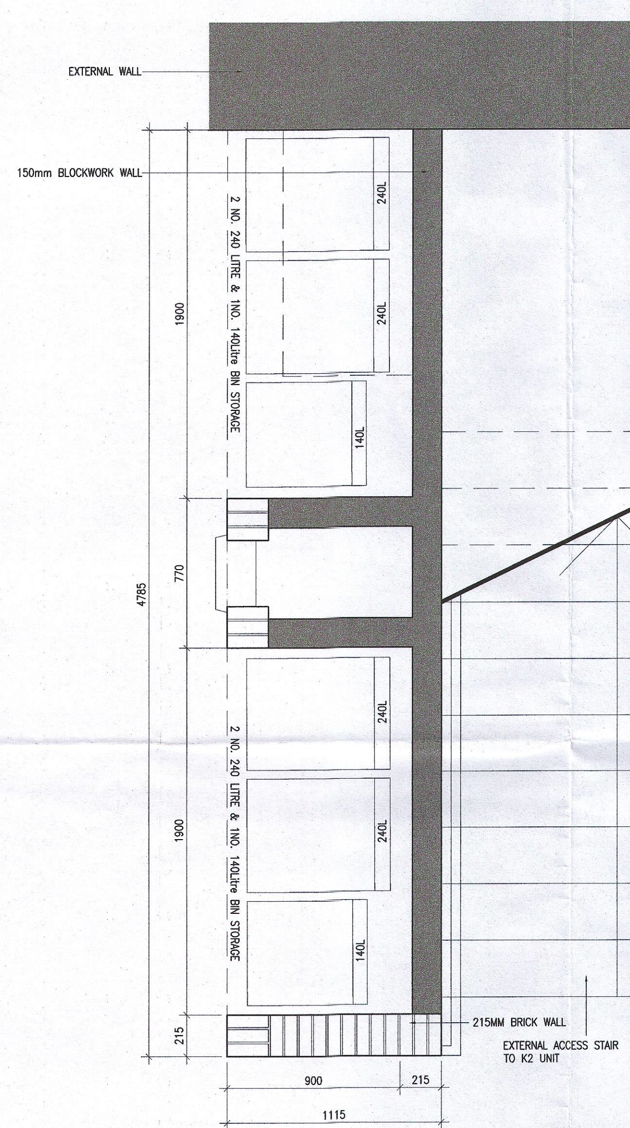
1 Bin store Type 4 Plan 704 Scale 1:20
