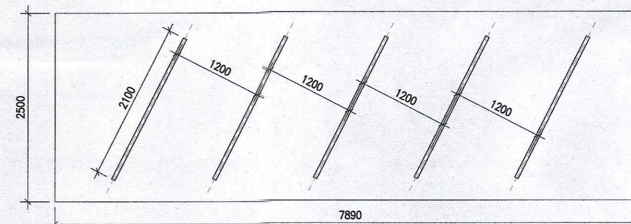
01 Proposed Cargo Parking Type 5 - Ground Plan P-702 1:500A1
