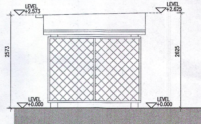
05 Proposed Cargo Bicycle Parking Type 3 - Elevation C P-702 1:500A1
