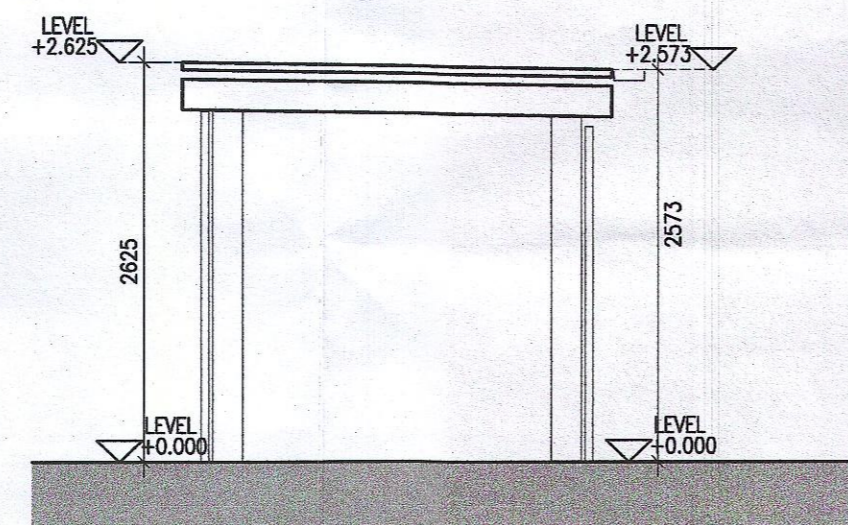
06 Proposed Cargo Bicycle Parking Type 3 - Section A-A P-702 1:500A1
