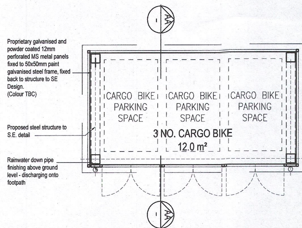
01 Proposed Cargo Bicycle Parking Type 3 - Ground Plan P-702 1:500A1
