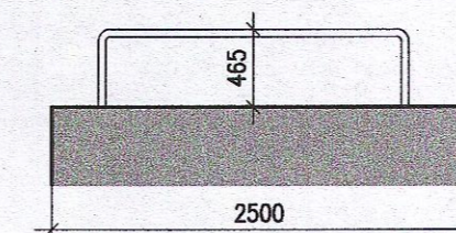
03 Proposed Cargo Parking Type 5 - Side Elevation P-702 1:500A1
