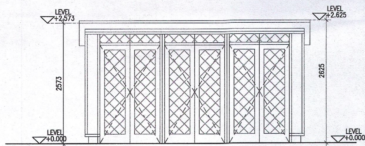
03 Proposed Cargo Bicycle Parking Type 3 - Elevation A P-702 1:500A1
