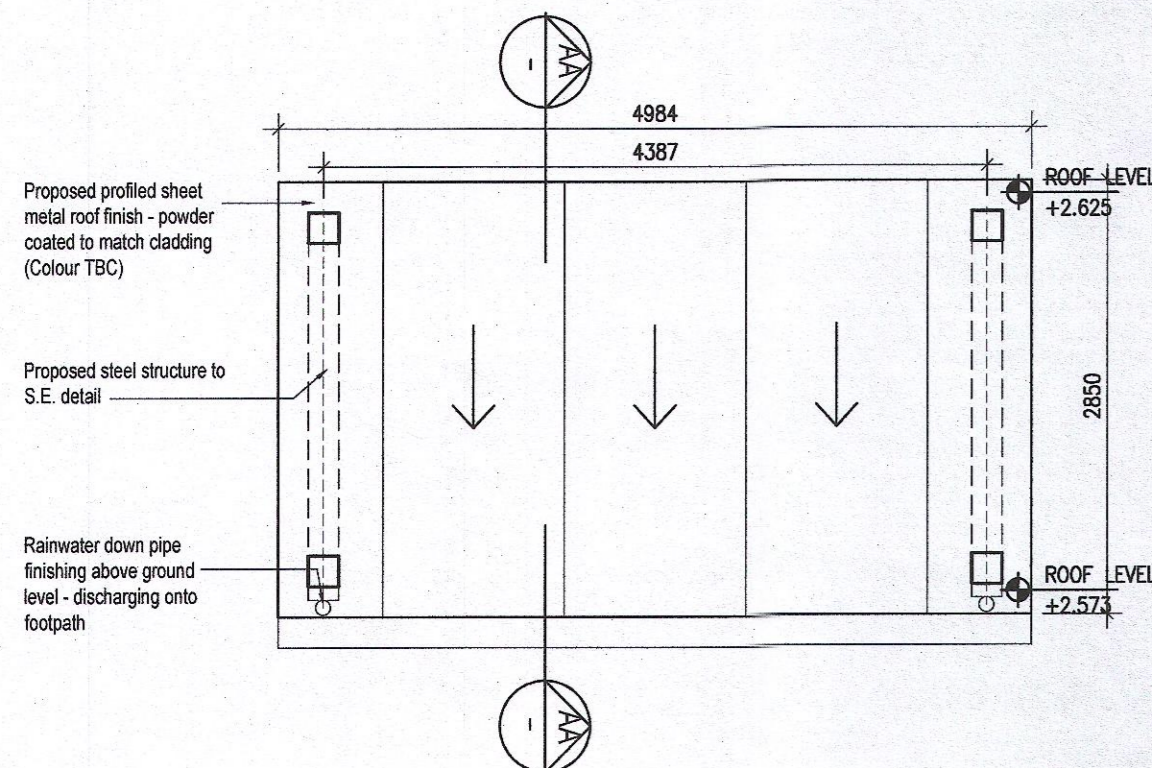
02 Proposed Cargo Bicycle Parking Type 3 - Roof Plan P-702 1:500A1
