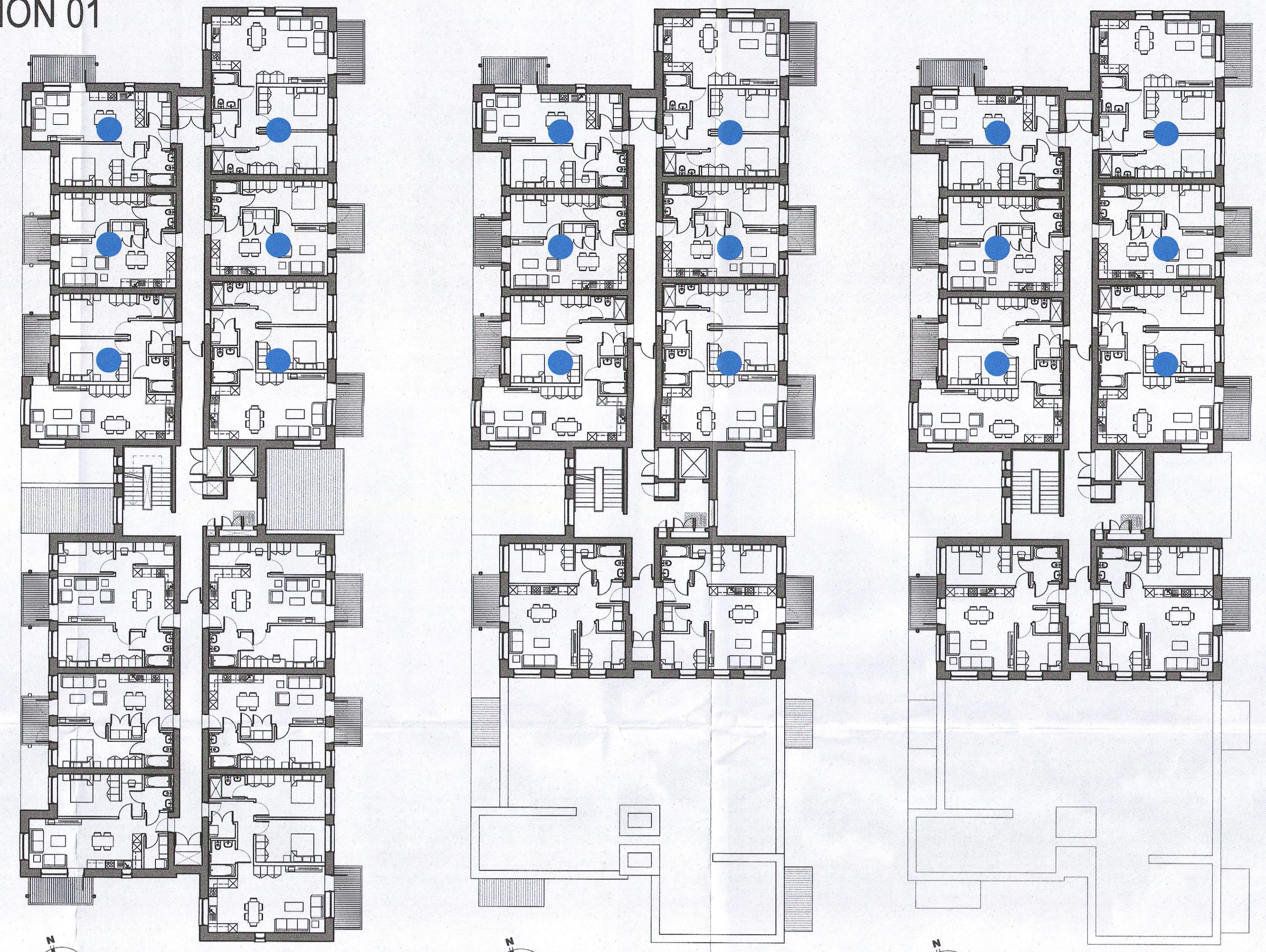
02 APARTMENTS - BLOCK 1- FIRST TO THIRD FLOOR (see drawings 6268-P-301,6268-P-302,6268-P-303)
