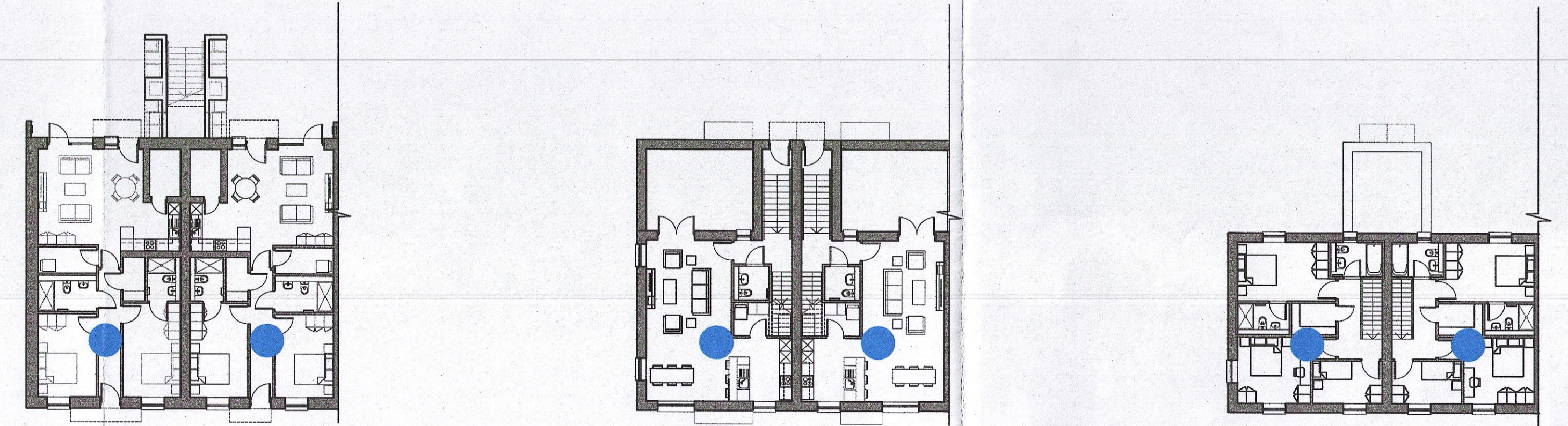
05 DUPLEX TYPES J1/K2 - GROUND PLAN (see drawings 6268-P-200,6268-P-202)
