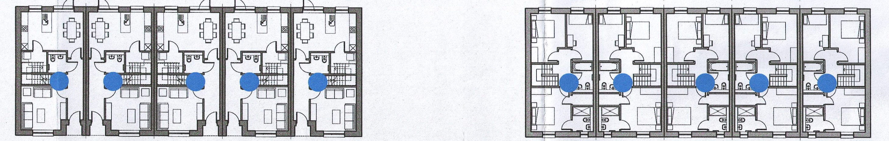
08 HOUSE TYPES E1 & E2 - GROUND PLAN (see drawings 6268-P-114,6268-P-115)
