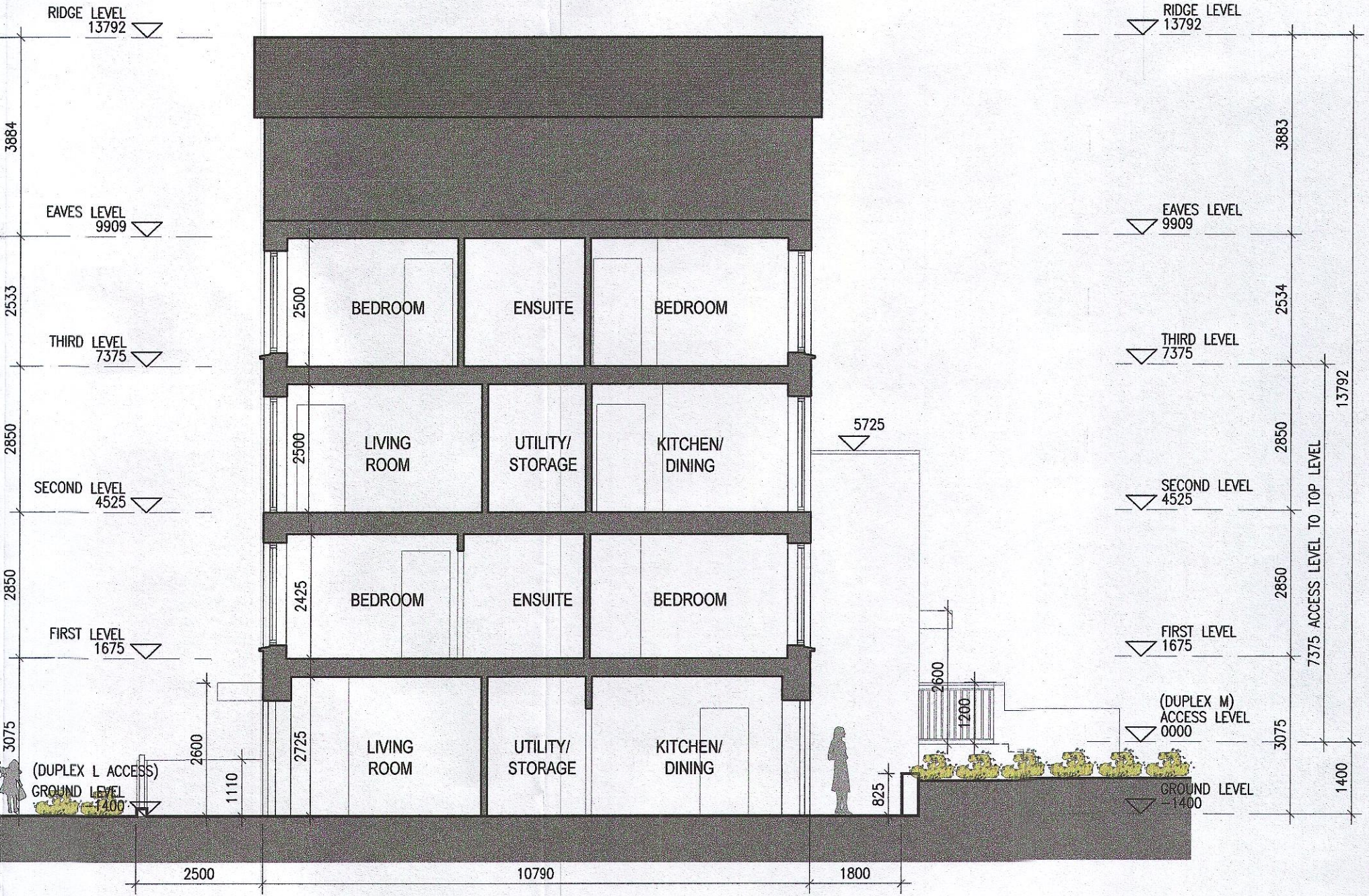
07 Typical Section B-B 1:100@A1
