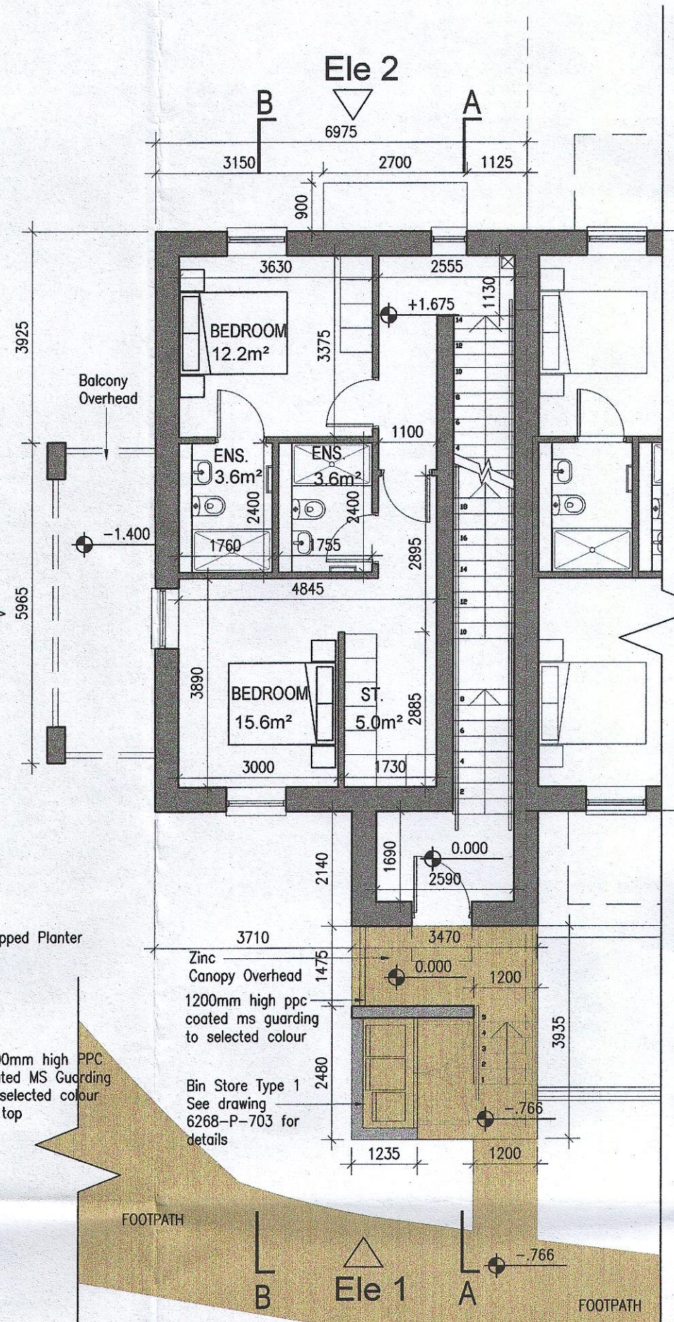
02 First Floor Plan
