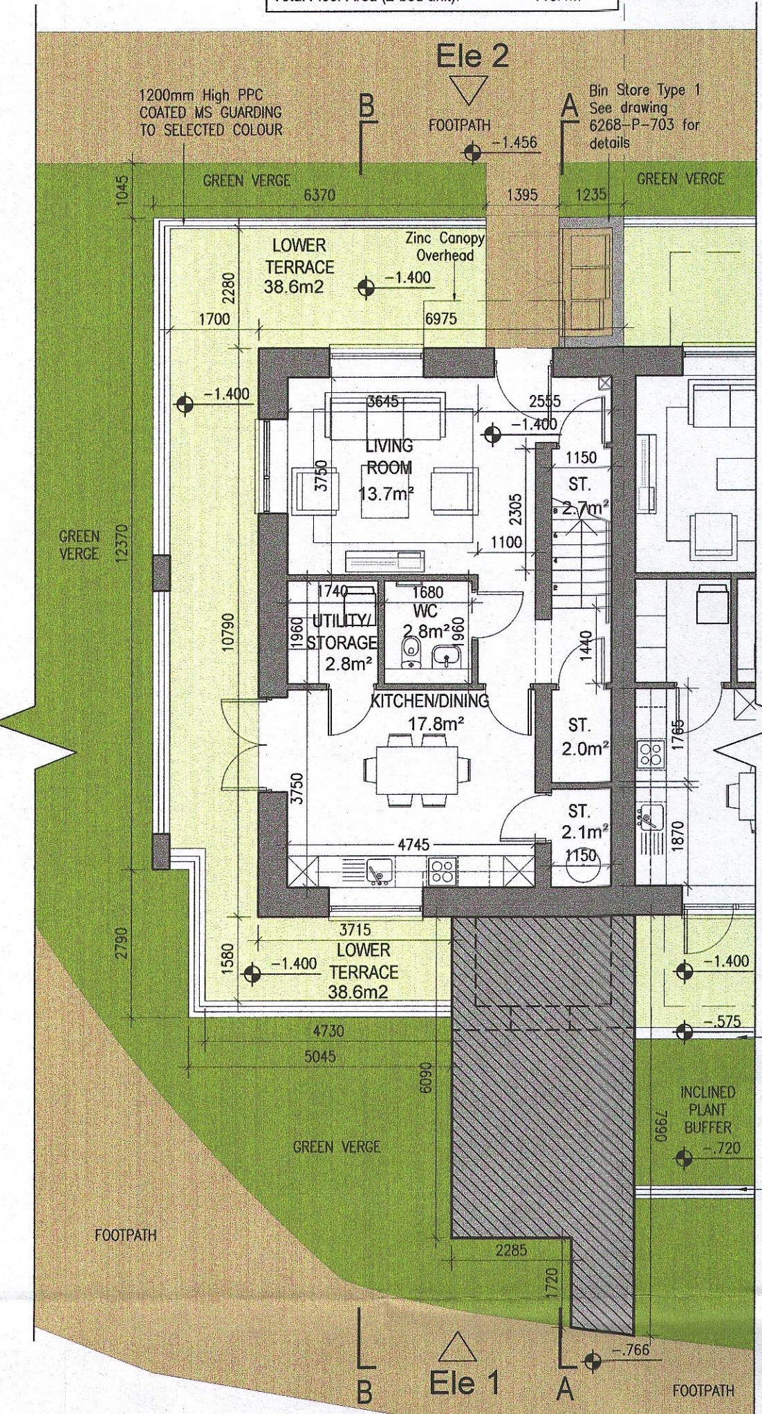
01 Ground Floor Plan
