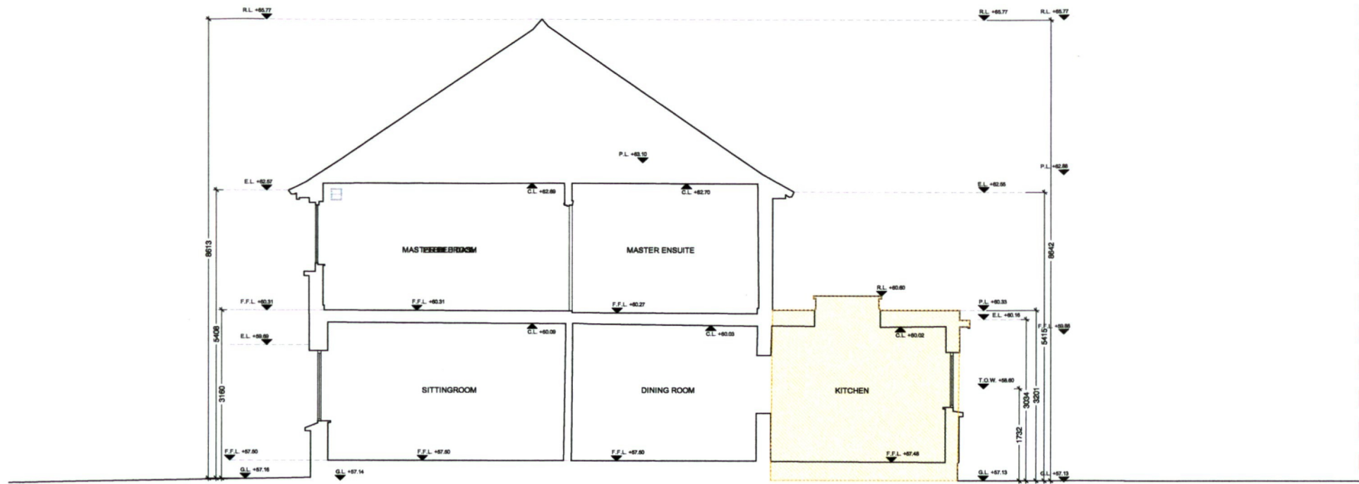
SECTION B-B / SIDE ELEVATION scale 1.100
