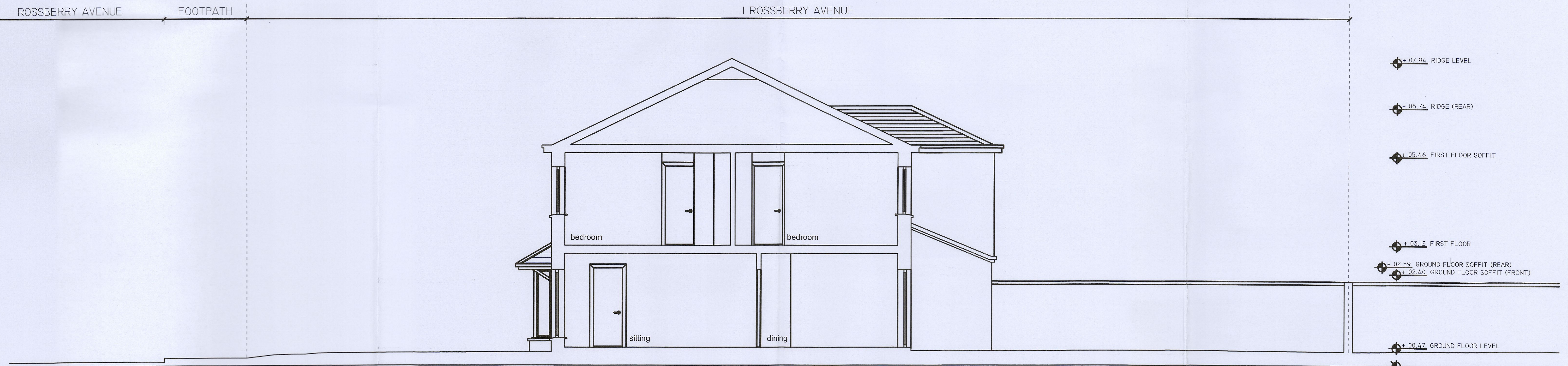
II.2 PROPOSED SECTION BB SCALE 1:100
