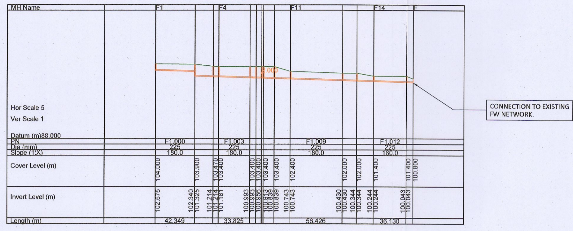
WASTE WATER NETWORK F1.000 - F1.013
