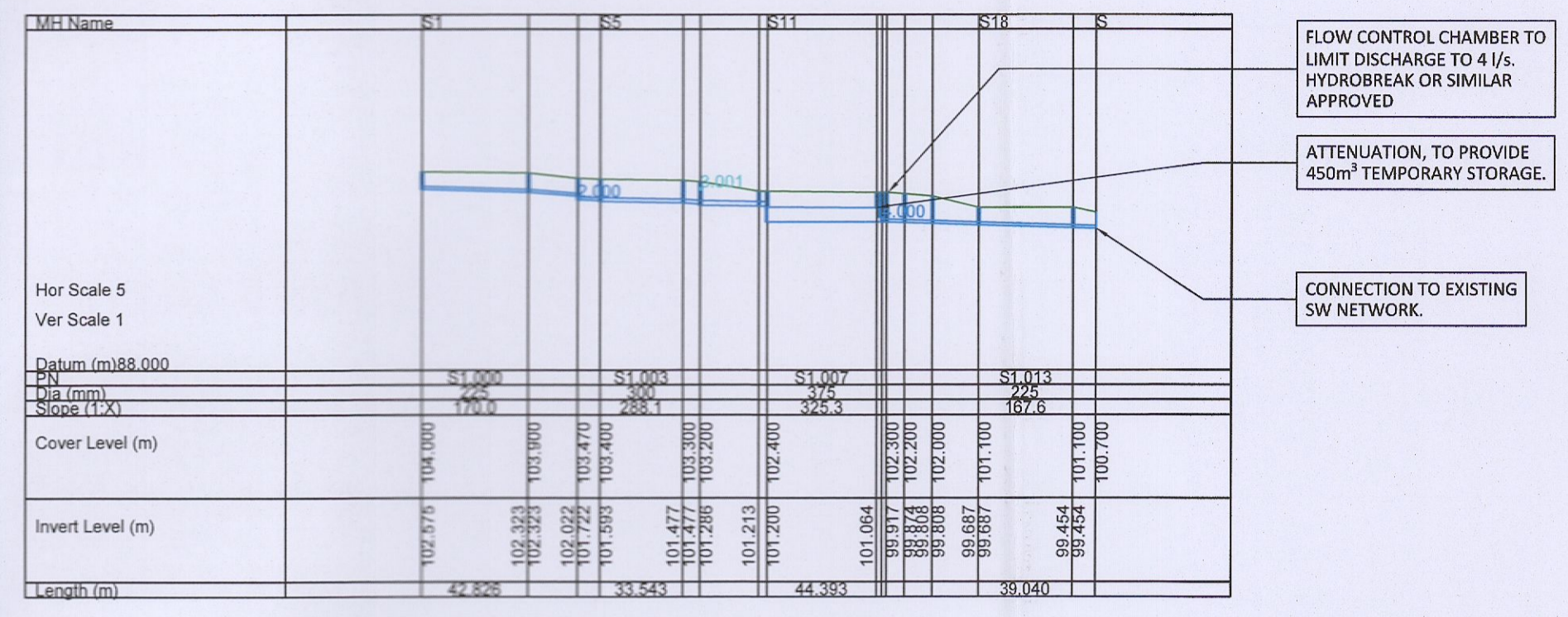
SURFACE WATER NETWORK S1.000 - S1.014
