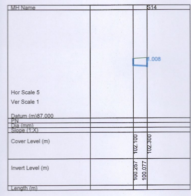
SURFACE WATER NETWORK S4.000
