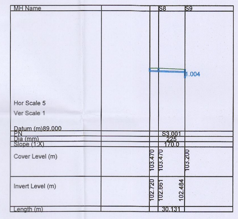
SURFACE WATER NETWORK S3.000 - S3.001
