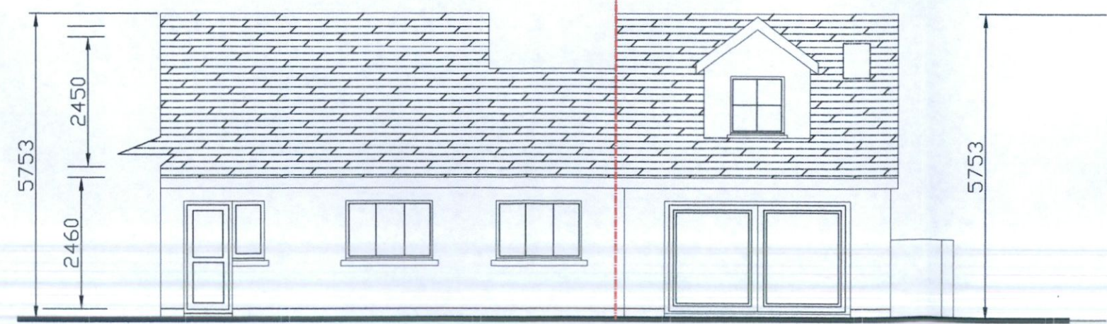
PROPOSED REAR ELEVATION / STREETSCAPE
