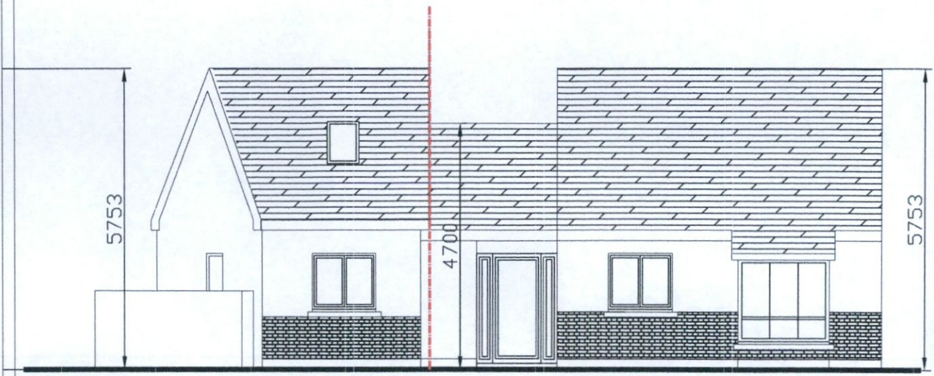
PROPOSED FRONT ELEVATION / STREETSCAPE
