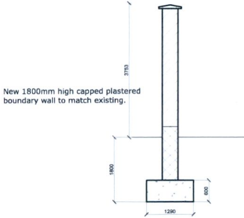
CROSS SECTION THRO. BOUNDARY WALL. Scale 1:50
