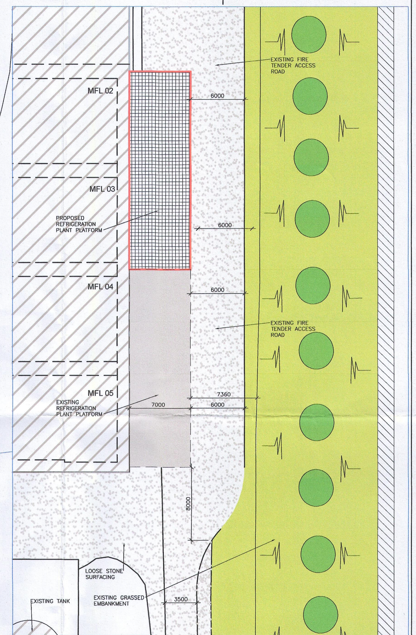
GANTRY PLATFORM SITE LAYOUT SCALE 1:200
