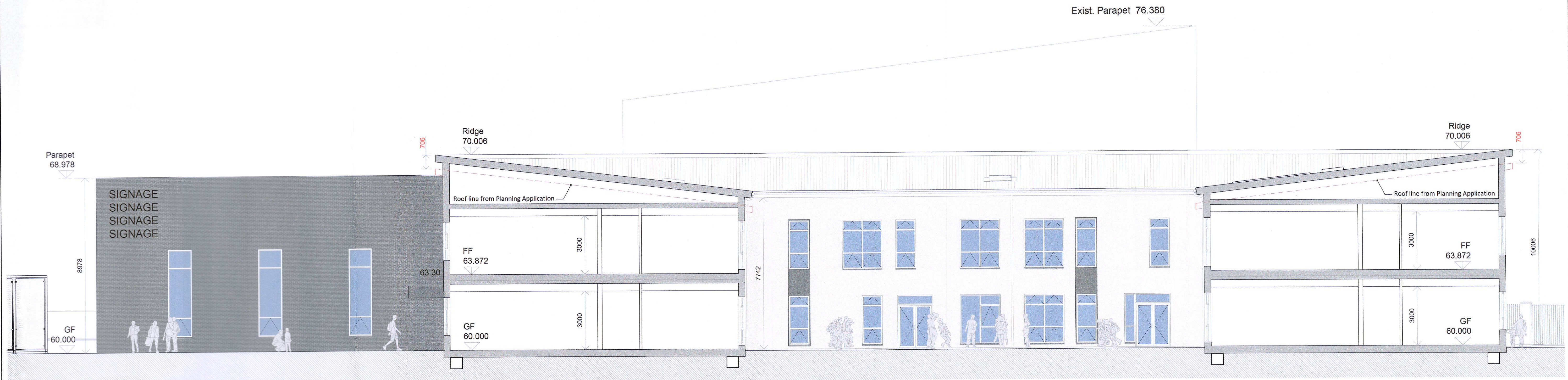
1 PROPOSED SECTION AA 1:100 @ A1
