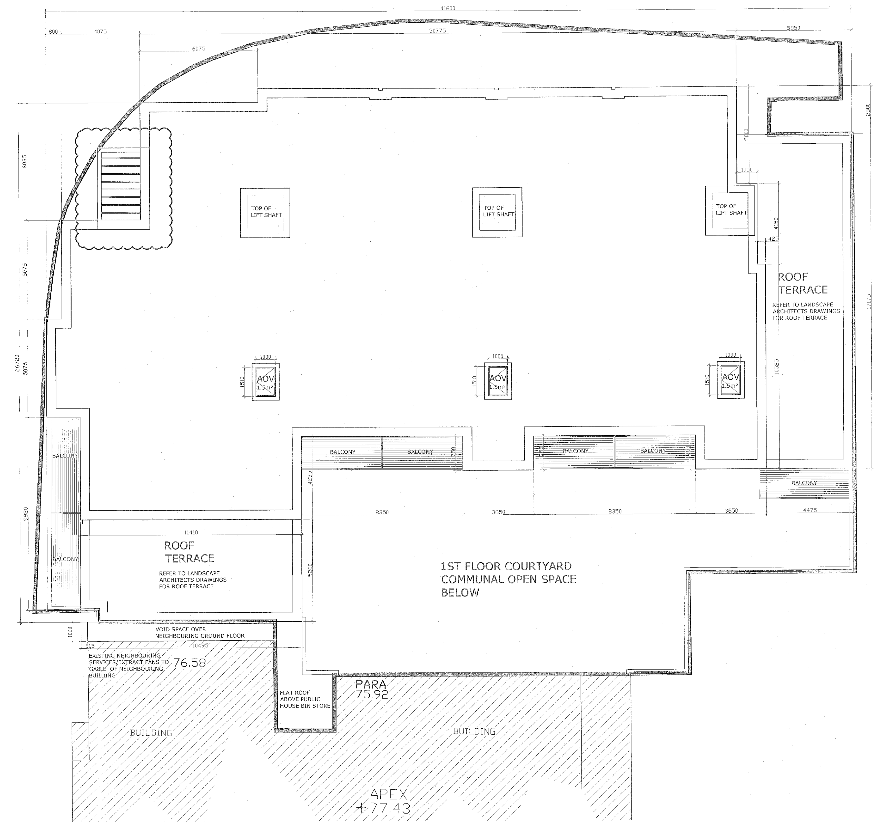
Proposed Roof Plan Scale 1:100
