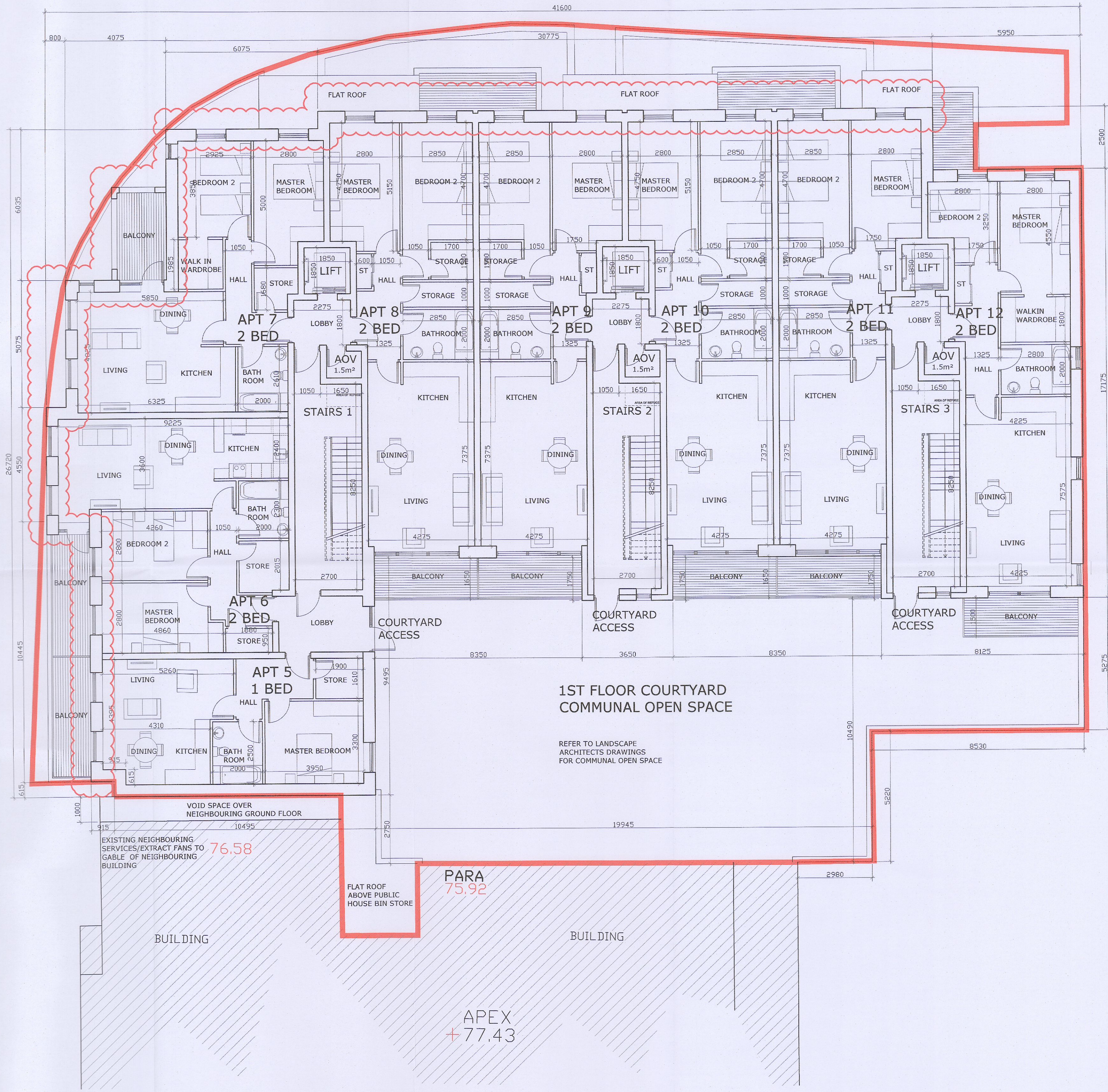
Proposed 1st Floor Plan Scale 1:100 A1, 1:200 A3
