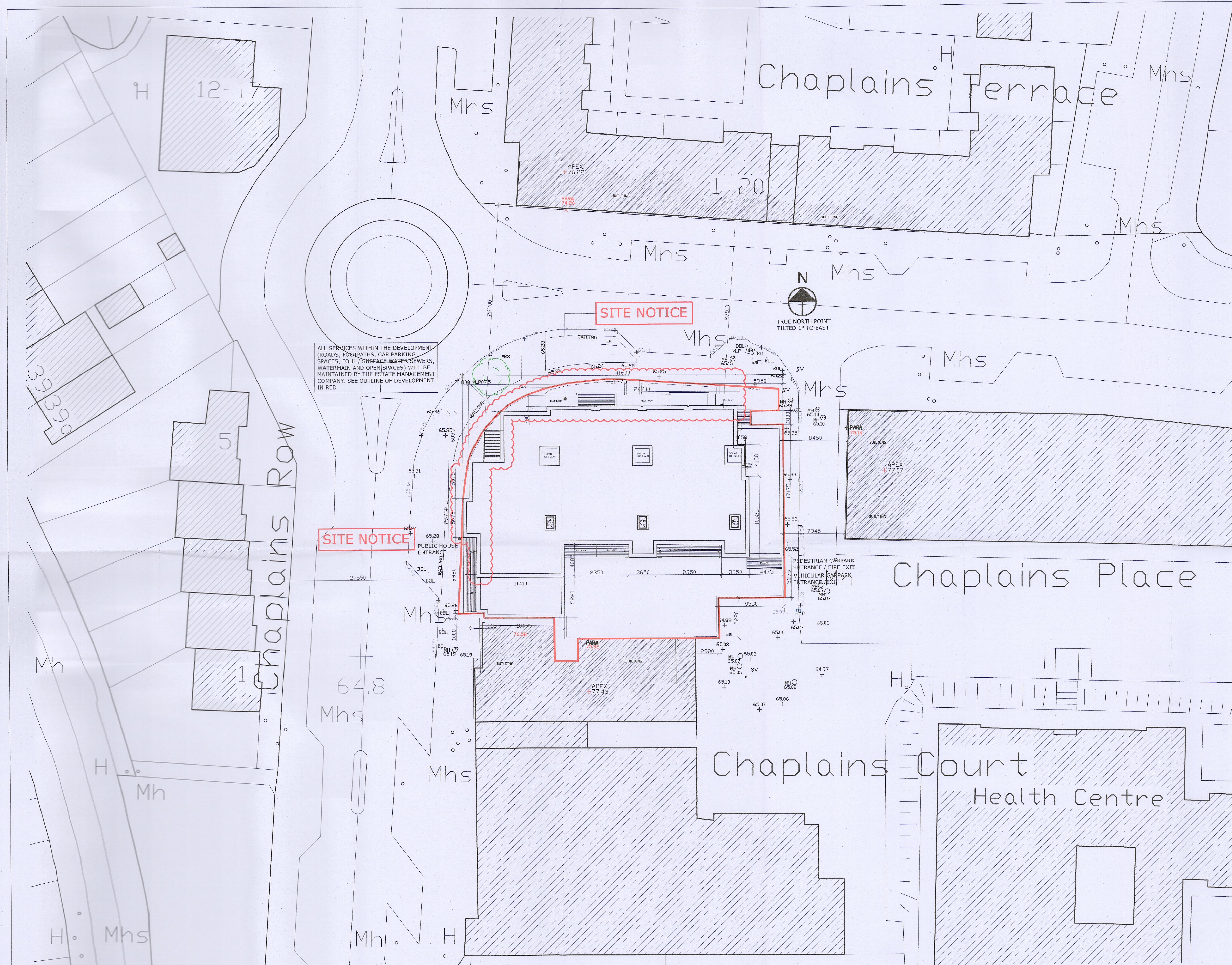
Proposed Site Plan Scale 1:250 A1, 1:500 A3
