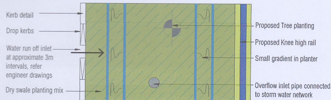
Section detail A; Plan View Scale 1: 50 @ A3
