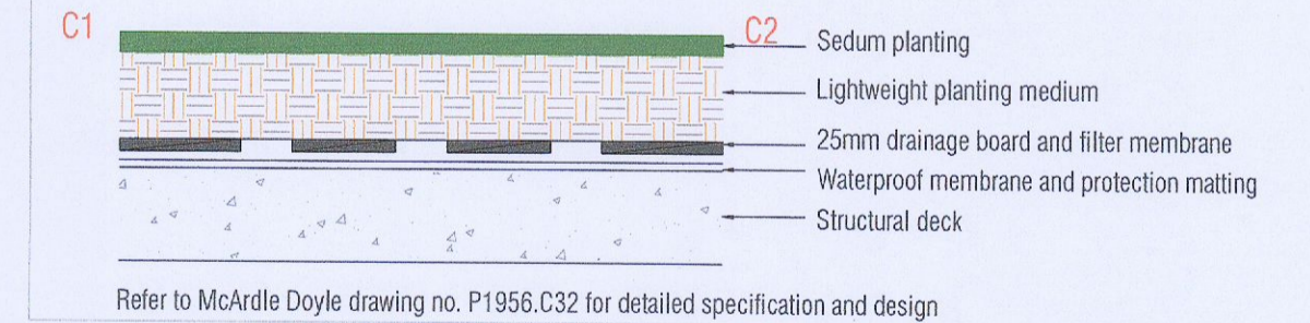
Detail C; Typical Green roof detail Scale 1: 20 @ A3
