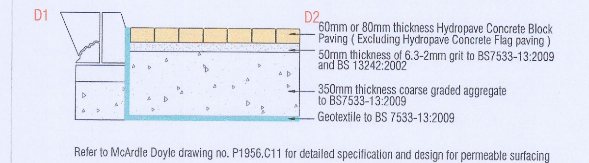
Detail D; Permeable paving Scale 1: 20 @ A3
