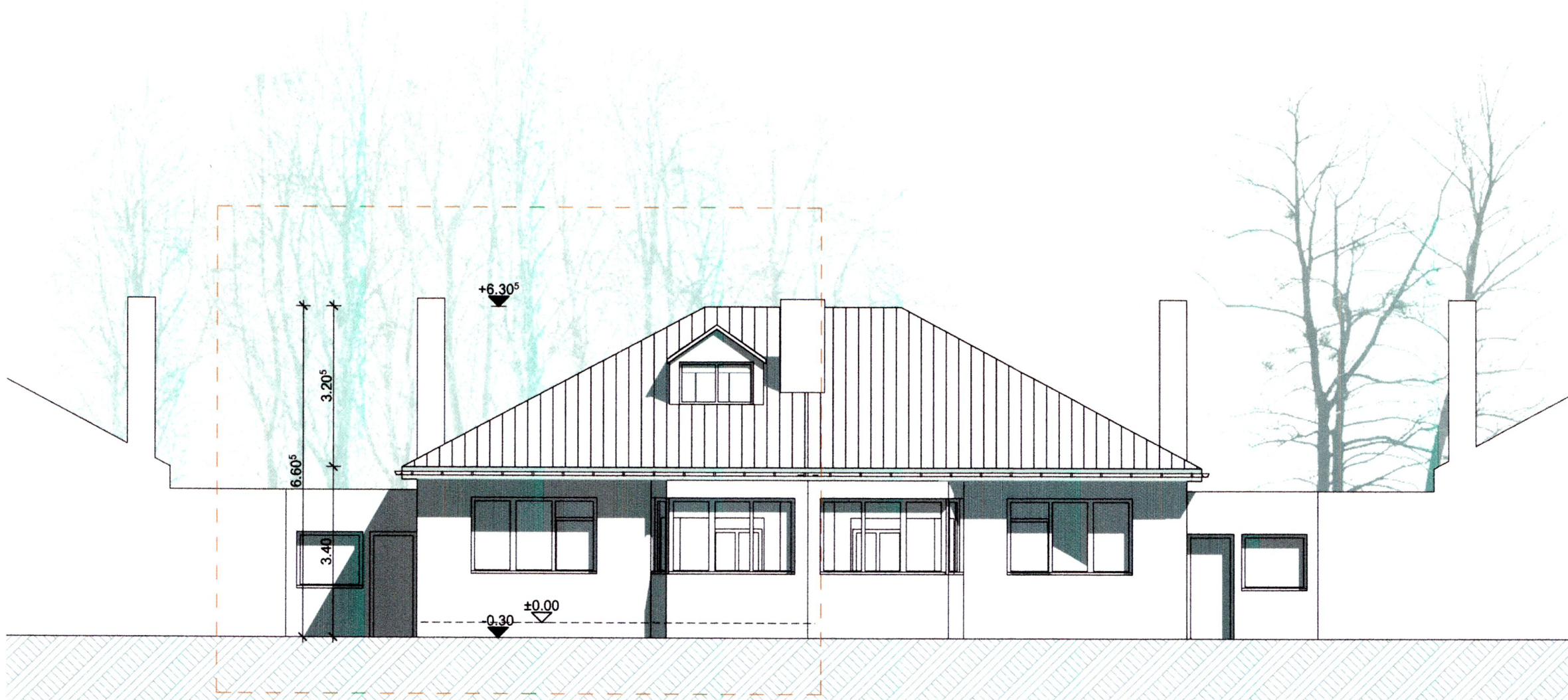
Existing Front Elevation_1:100
