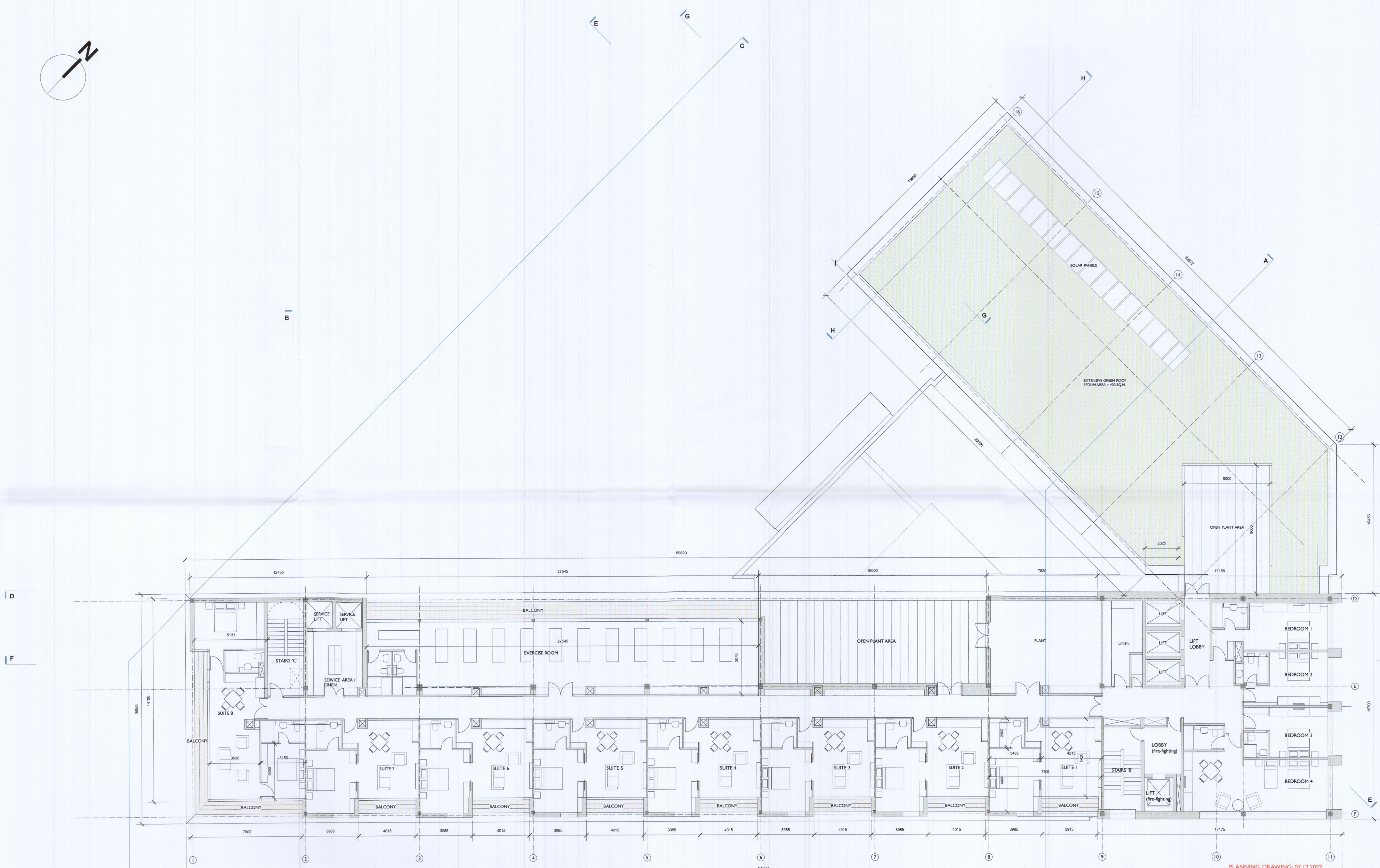
Level 6 plan 8 SUITES & 4 No. BEDROOMS 980 sq.m.
