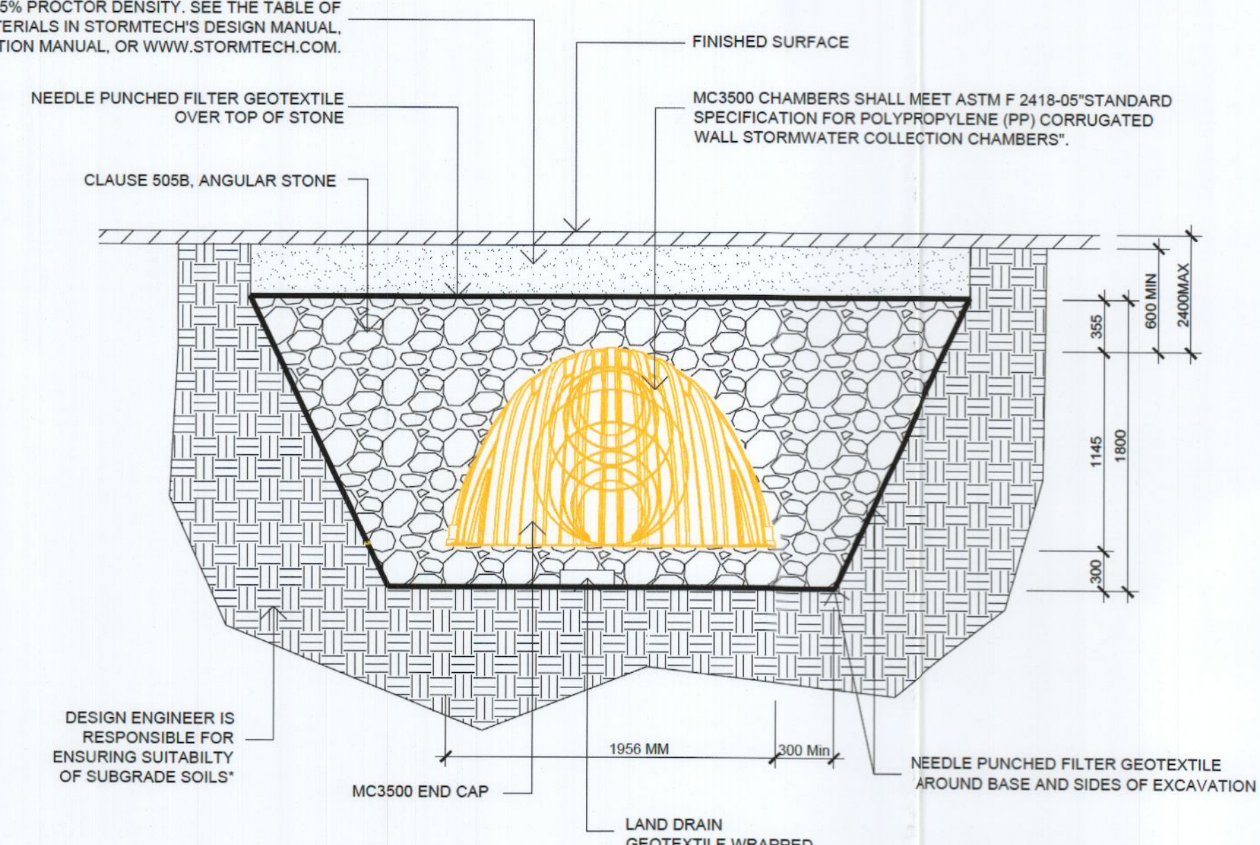
STORMTECH CHAMBER CROSS SECTION DETAIL A-A not to scale
