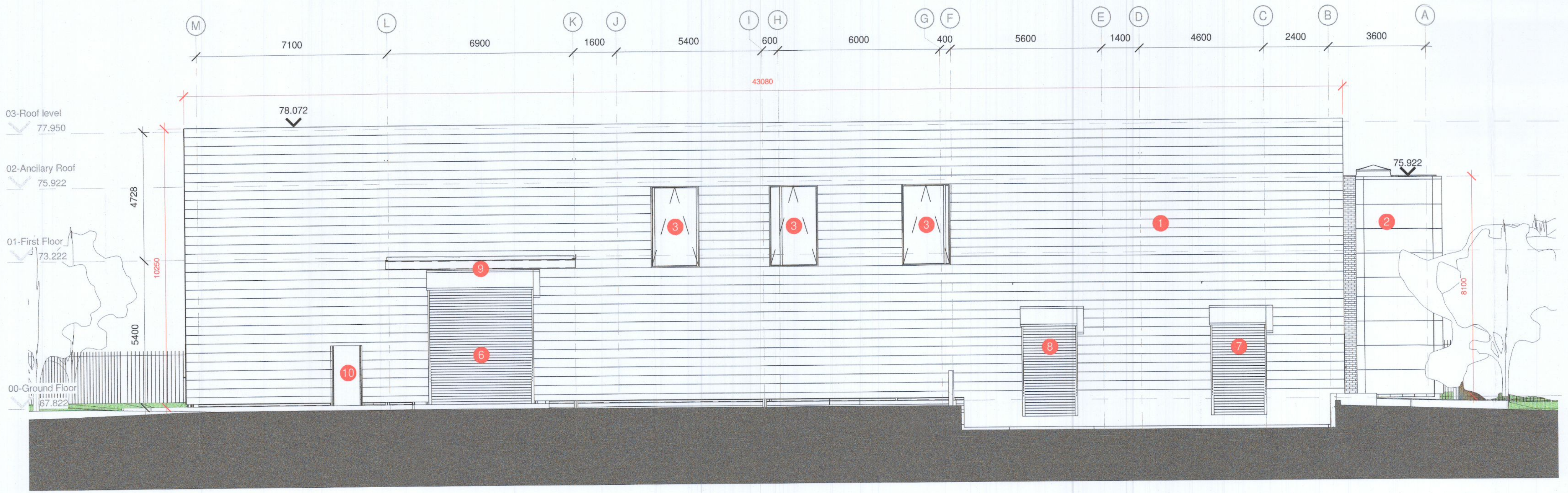
1 6507 Existing East Elevation 1 : 100
